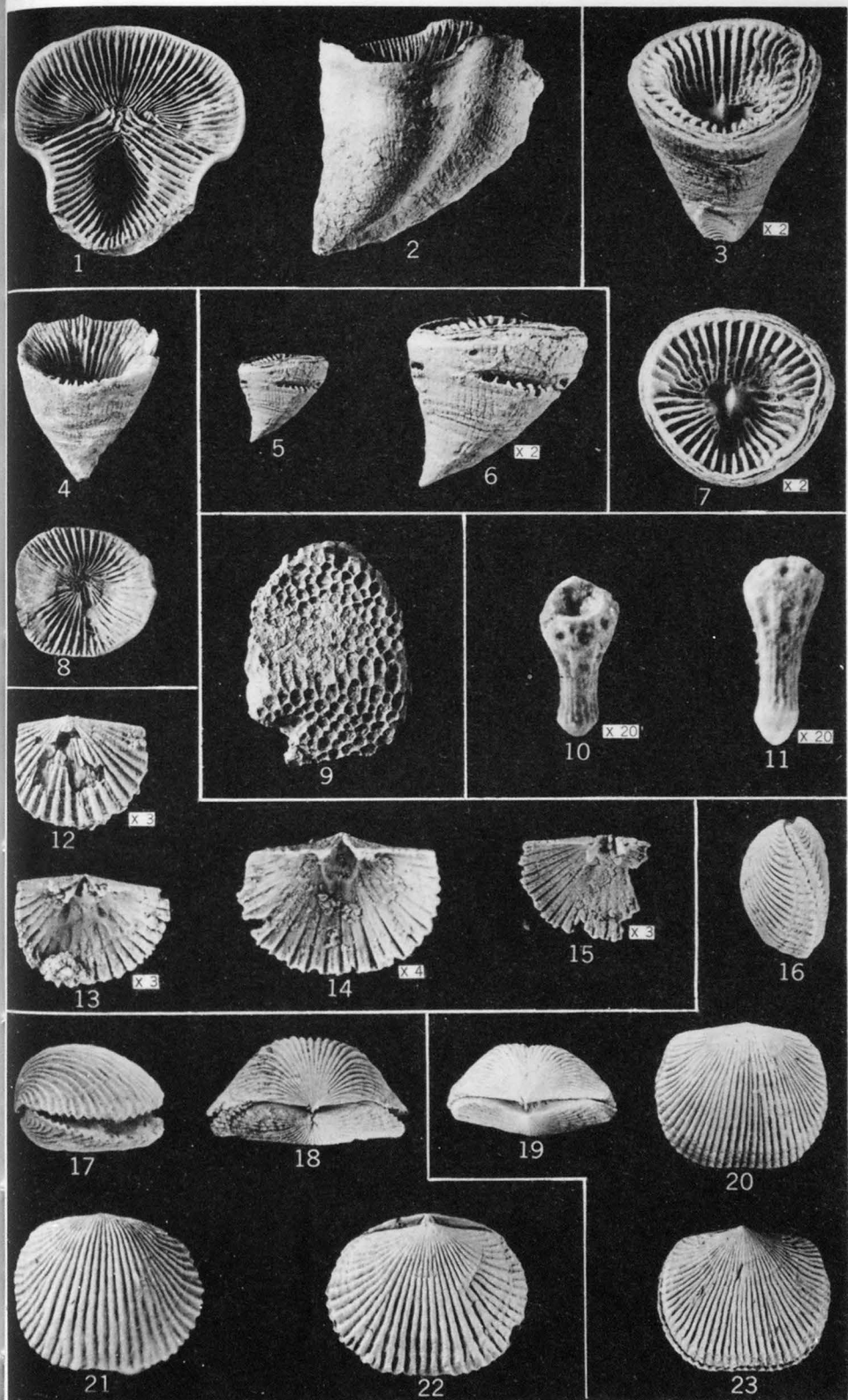
CORALS, BRYOZOAN, AND BRACHIOPODS (ORTHOCEA), BIGHORN AND RED RIVER FORMATIONS
