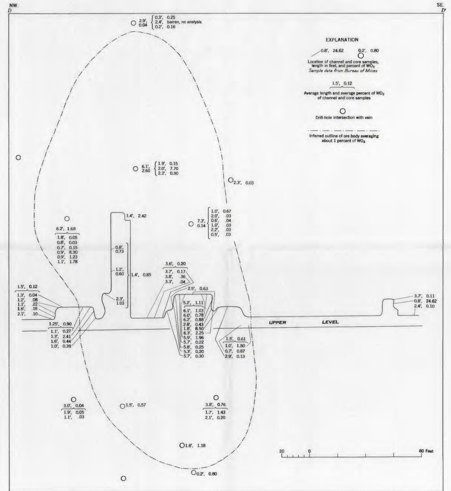
LONGITUDINAL PROJECTION OF MAIN WORKINGS IN LINDEBORG SHEAR ZONE, SHOWING DISTRIBUTION OF SCHEELITE, RIVERSIDE MINE (1942), HYDER DISTRICT, ALASKA
