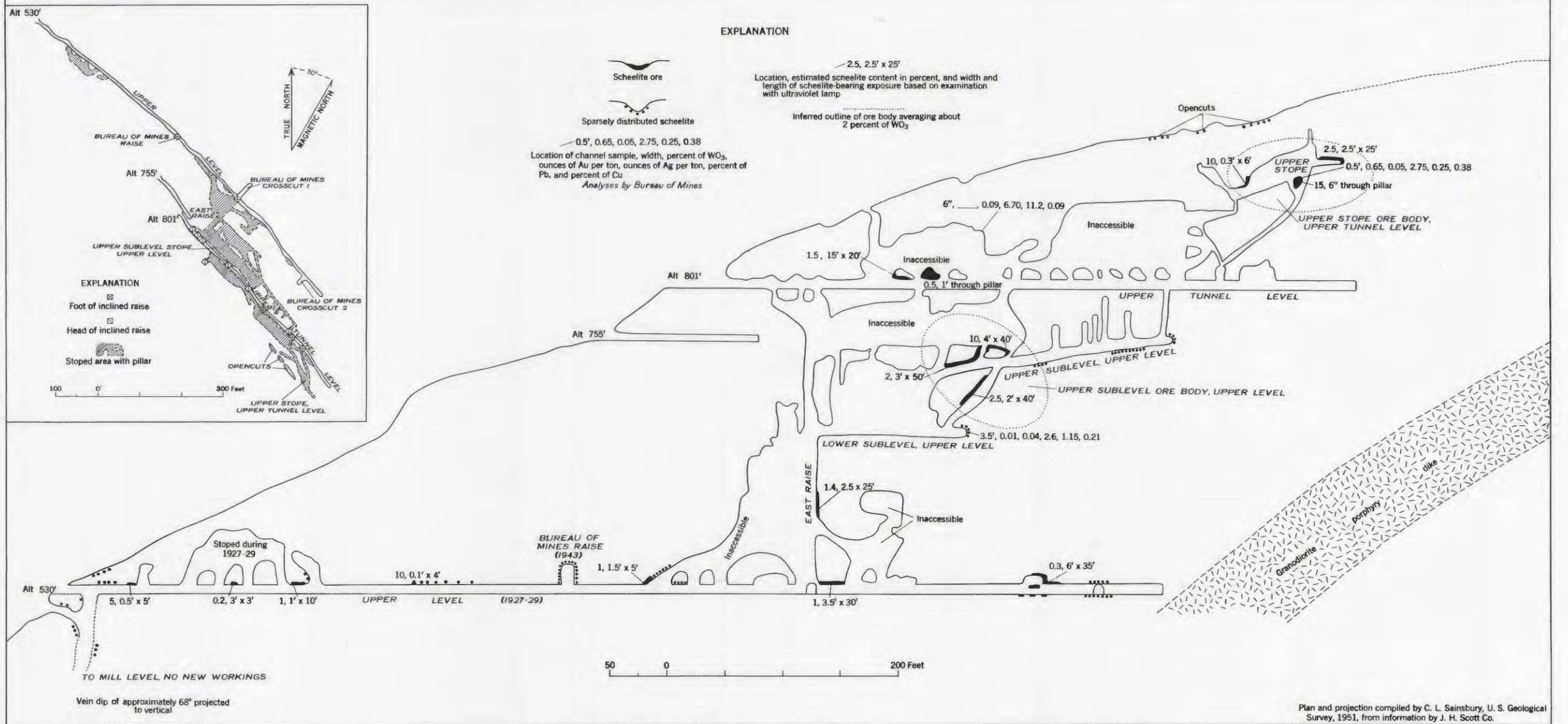
MAP AND LONGITUDINAL PROJECTION OF UPPER LEVELS, RIVERSIDE MINE, HYDER DISTRICT, ALASKA
