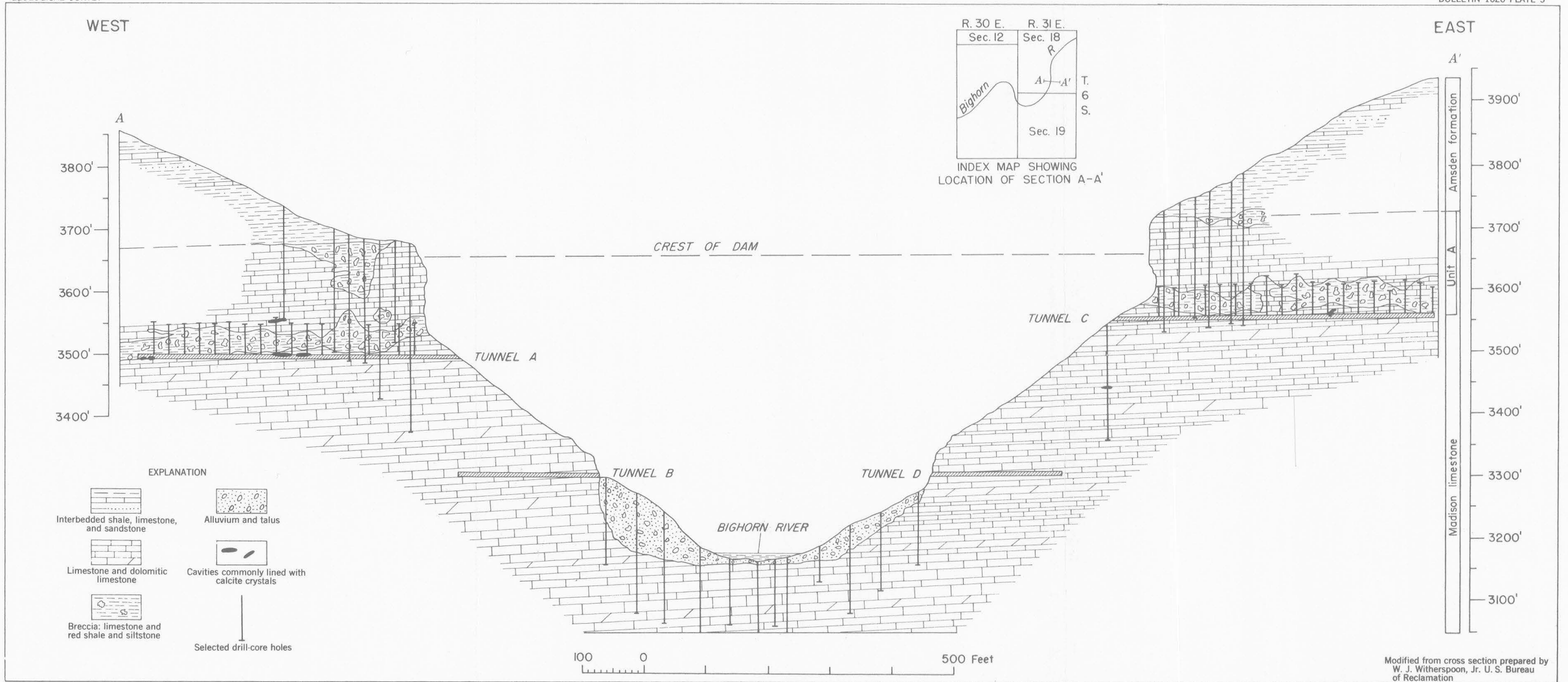
CROSS SECTION OF YELLOWTAIL DAM SITE, MONTANA. DOWNSTREAM VIEW SHOWING BRECCIATION IN UPPER MEMBER (UNIT A) OF THE MADISON LIMESTONE AS INTERPRETED FROM SELECTED DRILL CORES
