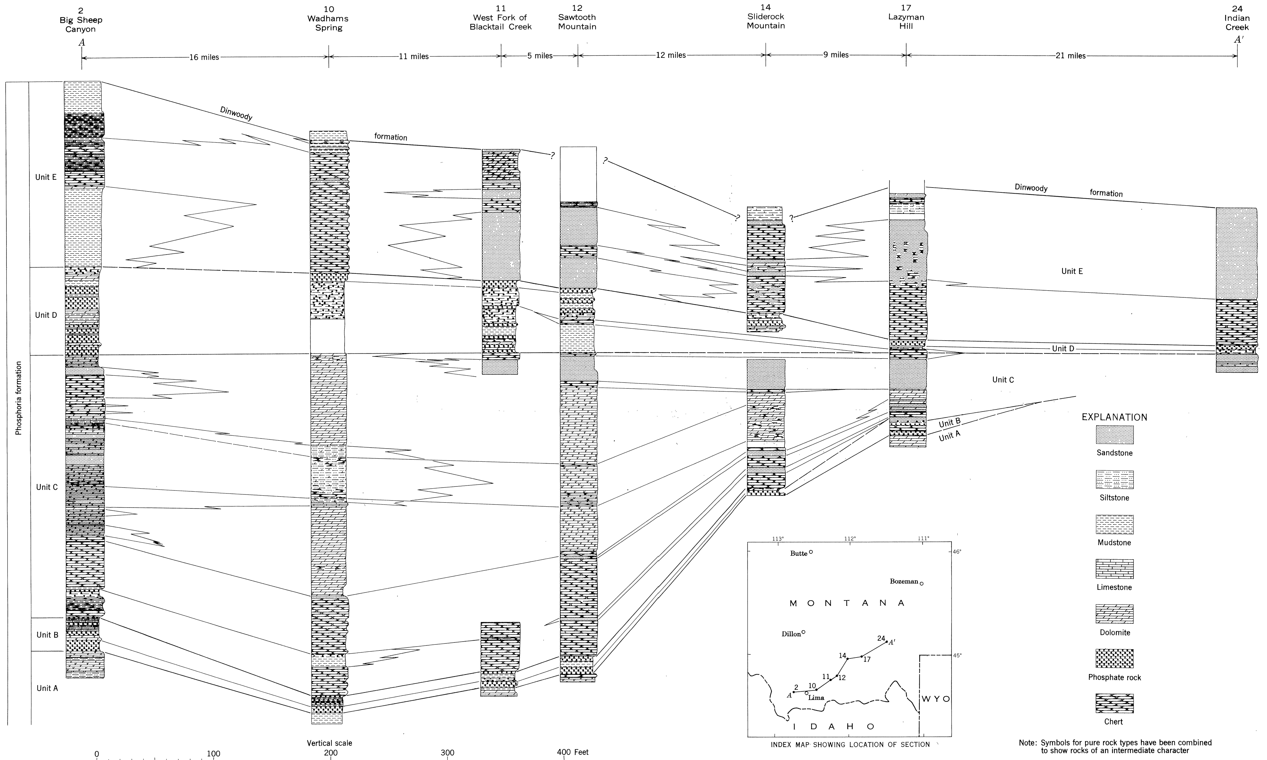
STRATIGRAPHIC SECTIONS SHOWING RELATIONS OF THE PHOSPHORIA FORMATION FROM BIG SHEEP CANYON TO TAYLOR FORK, MONTANA
