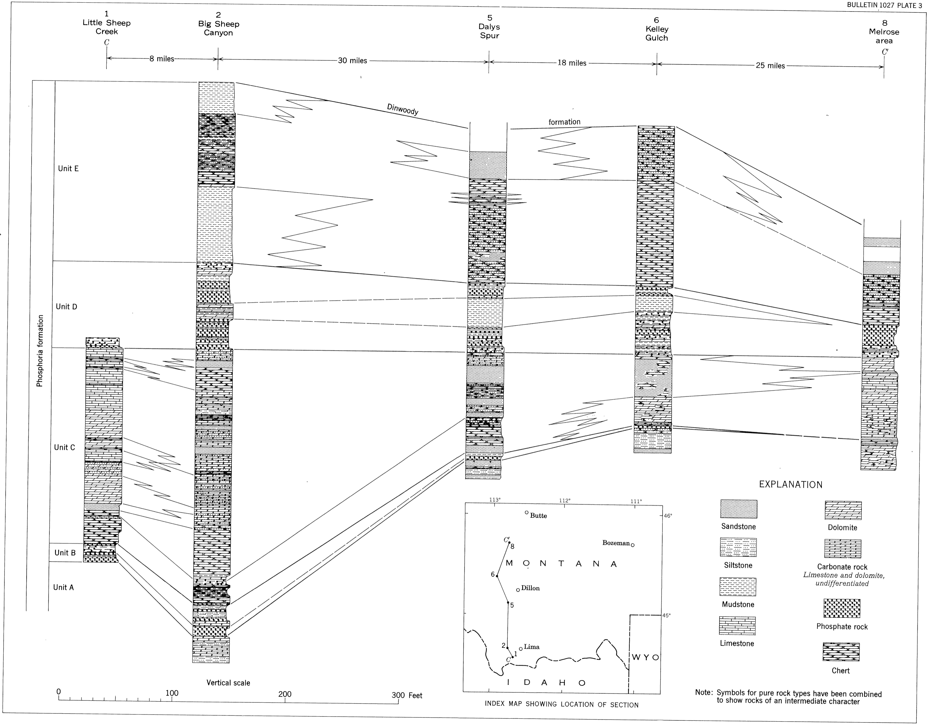
STRATIGRAPHIC SECTIONS SHOWING RELATIONS OF THE PHOSPHORIA FORMATION FROM LITTLE SHEEP CREEK TO MELROSE, MONTANA
