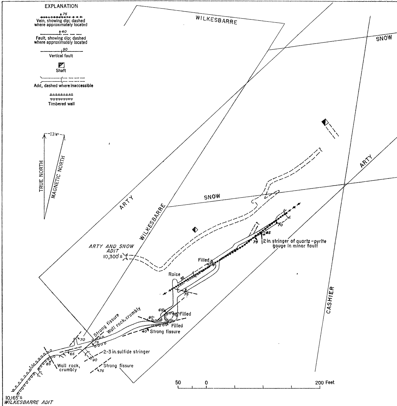
PLAN OF THE WILKESBARRE MINE, ALONG ARTY AND SNOW VEIN, ST. KEVIN DISTRICT, LAKE COUNTY, COLORADO
