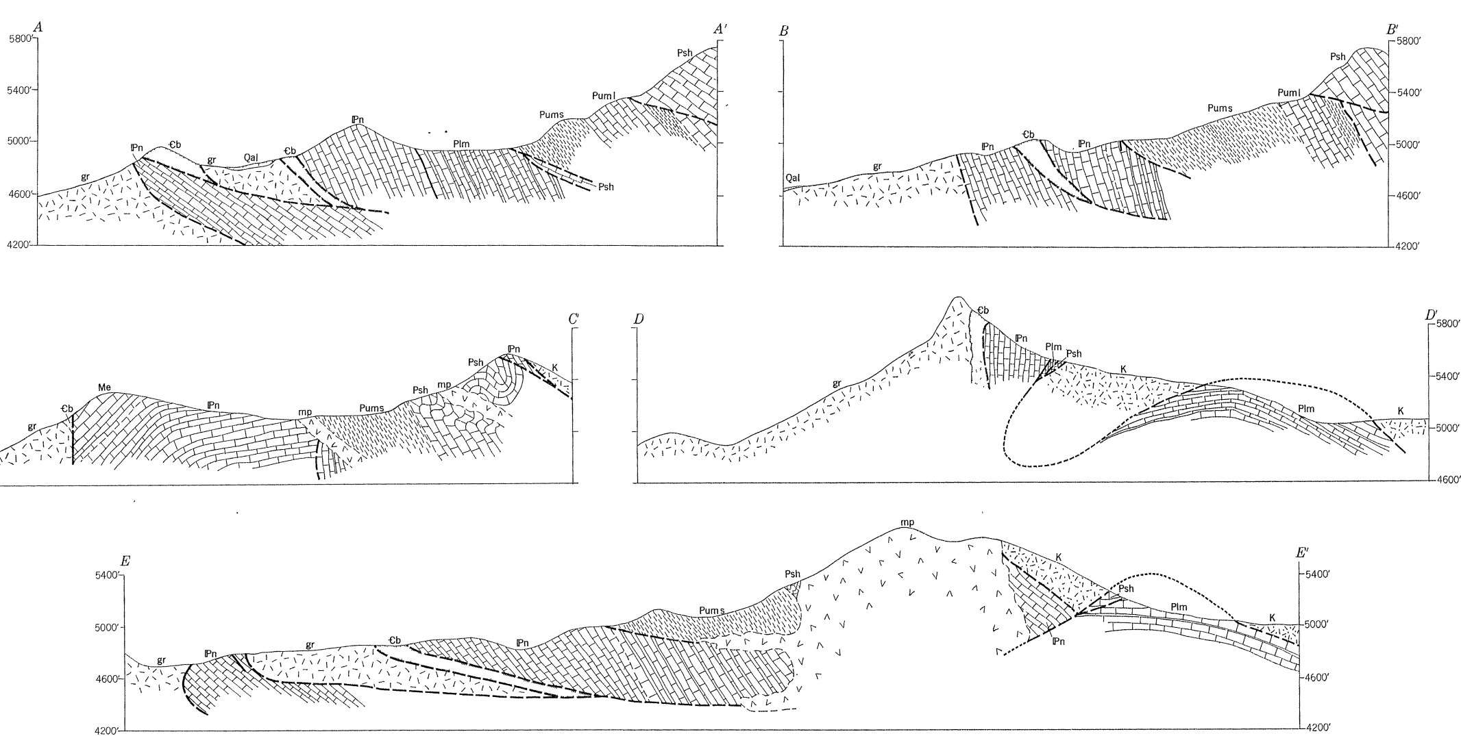
GENERALIZED GEOLOGIC MAP AND SECTIONS OF THE AREAS ADJACENT TO THE ROSEMONT LEASE AND THE LEADER, COPPER WORLD, AND NARRAGANSETT MINES, HELVETIA MINING DISTRICT, PIMA COUNTY, ARIZONA
