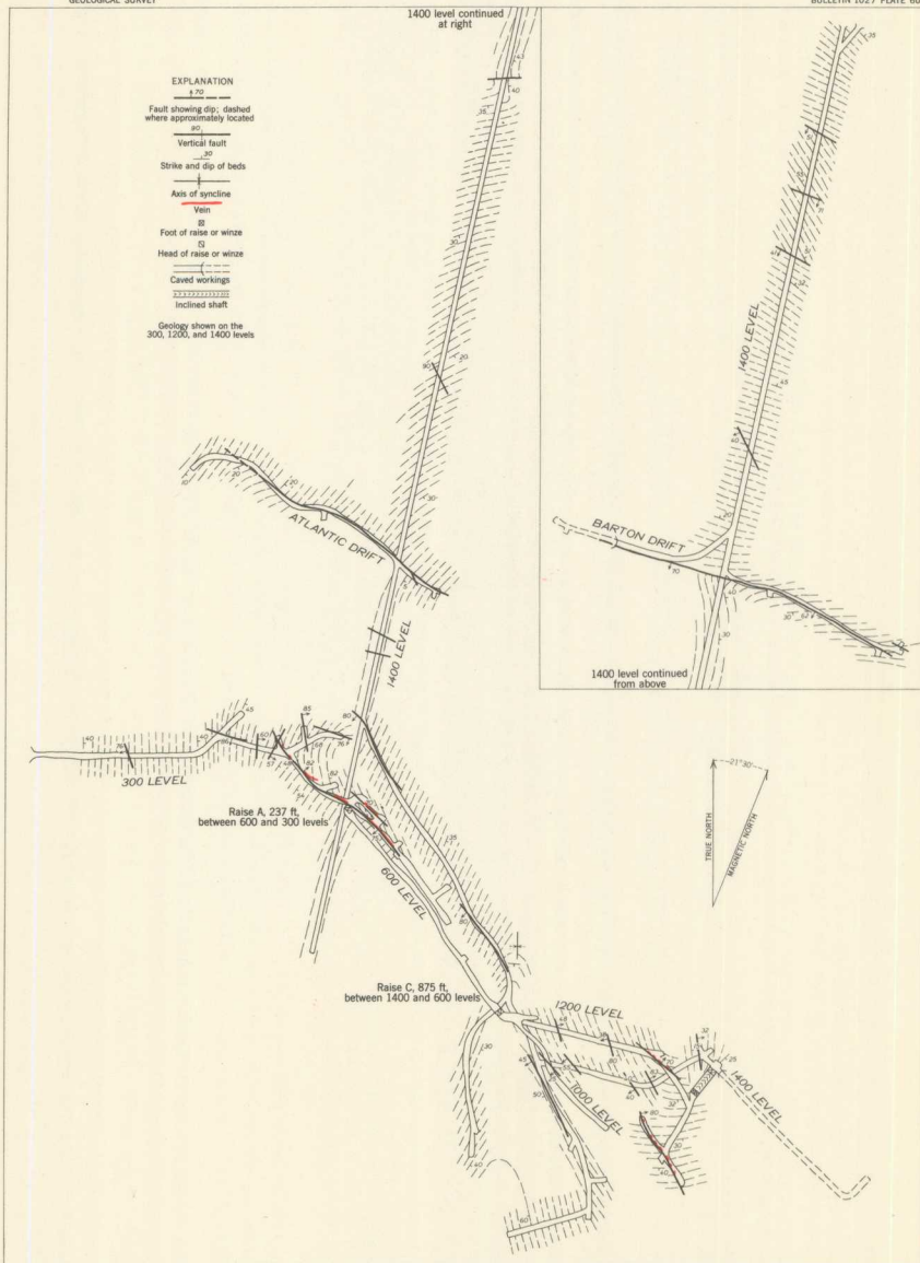
GEOLOGICAL MAP OF WORKINGS OF THE MONARCH MINE, SHOSHONE COUNTY, IDAHO
