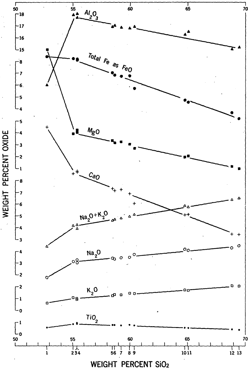
FIGURE 42.—Silica-variation diagram of rocks of Little Sitkin Island. Lines drawn by inspection. Analyses numbers correspond with column numbers in table 2.
