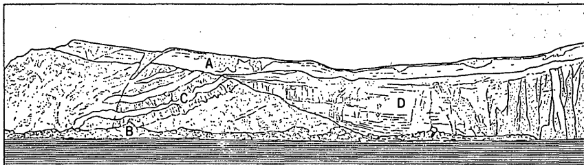
FIGURE 41.—Diagrammatic view of unconformity on Sitkin Point looking northwest. Drawn from a photograph. A , ash and turf mantle; B , boulder beach; C , massive and iron stained breccia layers of subaerial flows of Williwaw Cove formation; D , horizontally bedded, vertically jointed tuffaceous graywacke of Sitkin Point formation.
