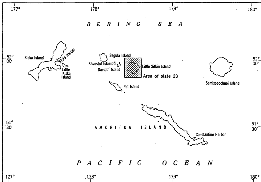
FIGURE 39.—Index map of the Aleutian Islands and land bordering the Bering Sea, showing location of the Rat Islands, and index map of the Rat Islands, showing location of Little Sitkin Island.
