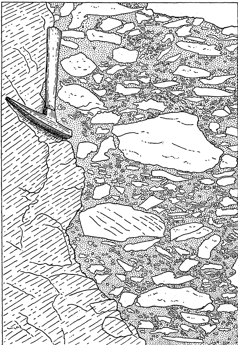
FIGURE 40.—Cliff exposure of tuff-breccia in the Sitkin Point formation as exposed in vertical face of "Caldera Two" scarp north of the 1,900-foot mountain. The boulders are allined parallel to bedding. Drawn from a photograph.
