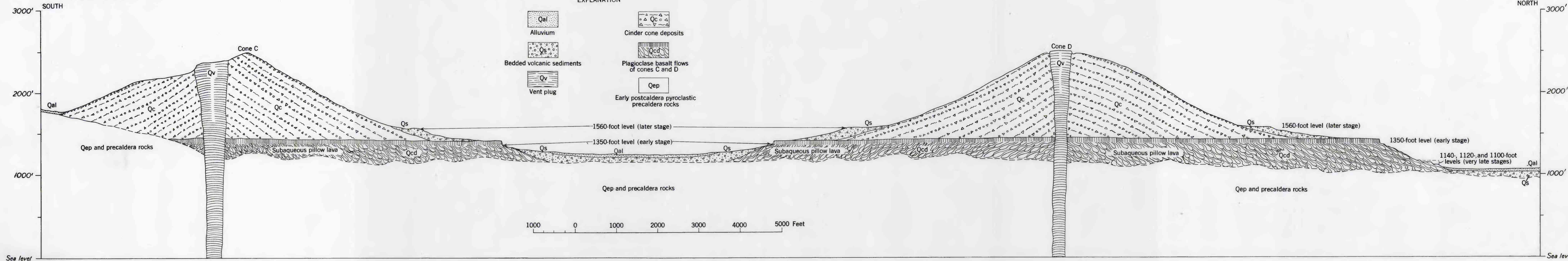
SECTION THROUGH CONES C AND D SHOWING DIFFERENT LAKE LEVELS AND RELATIONS BETWEEN ROCKS CONTEMPORANEOUS WITH CALDERA LAKE, UMNAK ISLAND, ALEUTIAN ISLANDS, ALASKA
