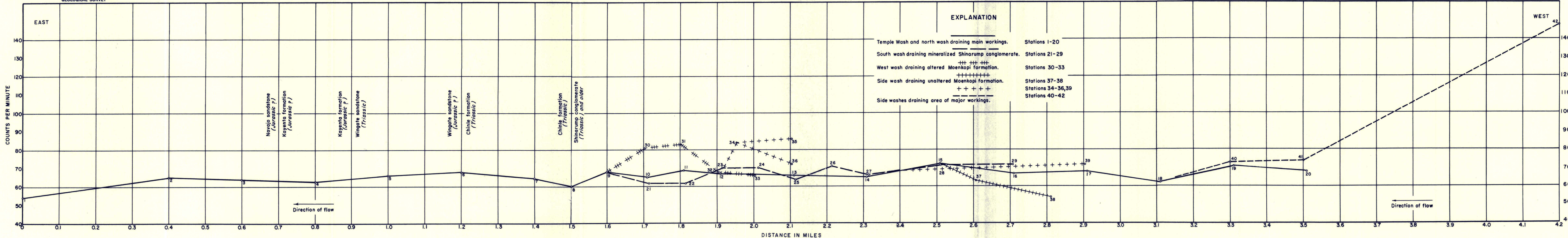
GRAPH SHOWING RADIOACTIVITY IN STREAM GRAVELS, TEMPLE MOUNTAIN AREA, SAN RAFAEL DISTRICT, EMERY COUNTY, UTAH
