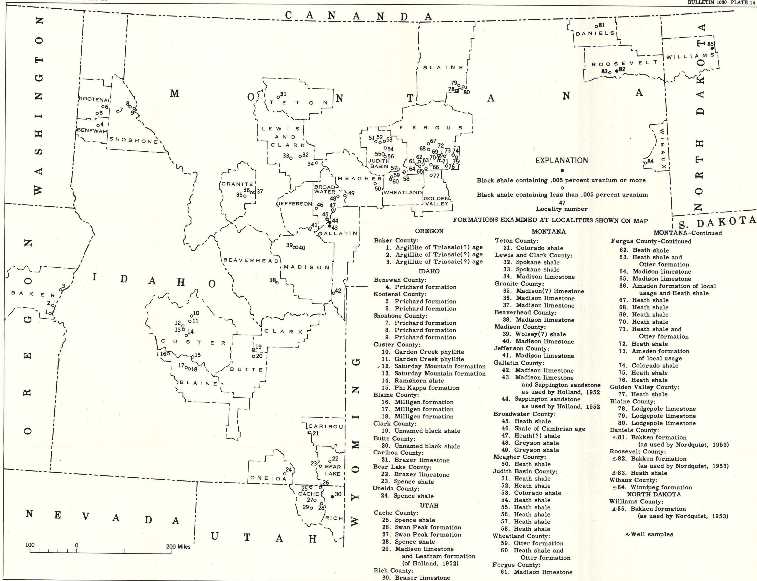
INDEX MAP SHOWING BLACK SHALE LOCALITIES EXAMINED FOR URANIUM, NORTHERN ROCKY MOUNTAINS AND GREAT PLAINS
