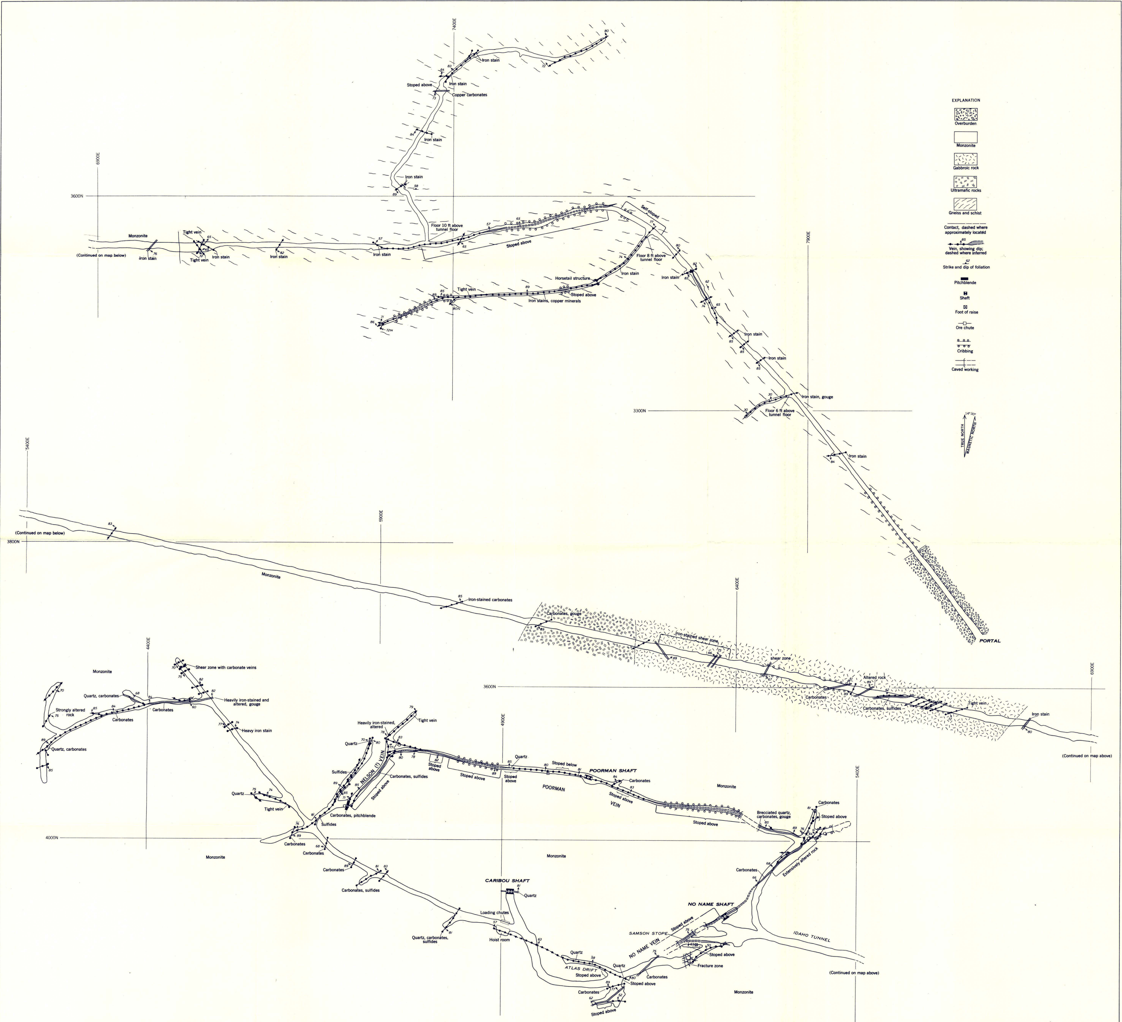
GEOLOGIC MAP OF THE 500 LEVEL AND THE IDAHO TUNNEL, CARIBOU MINE, BOULDER COUNTY, COLORADO
