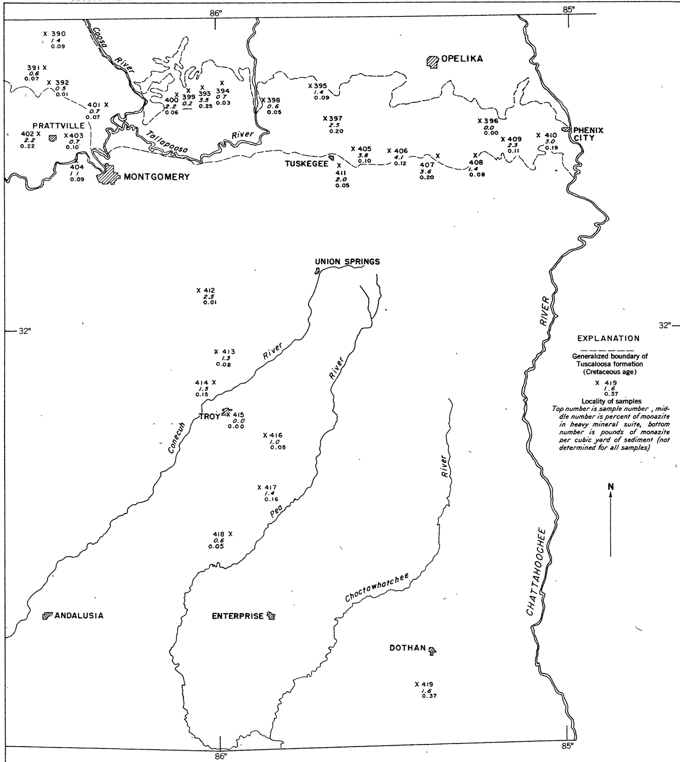
LOCATION AND MONAZITE CONTENT OF SAMPLES IN PART OF THE COASTAL PLAIN IN ALABAMA
