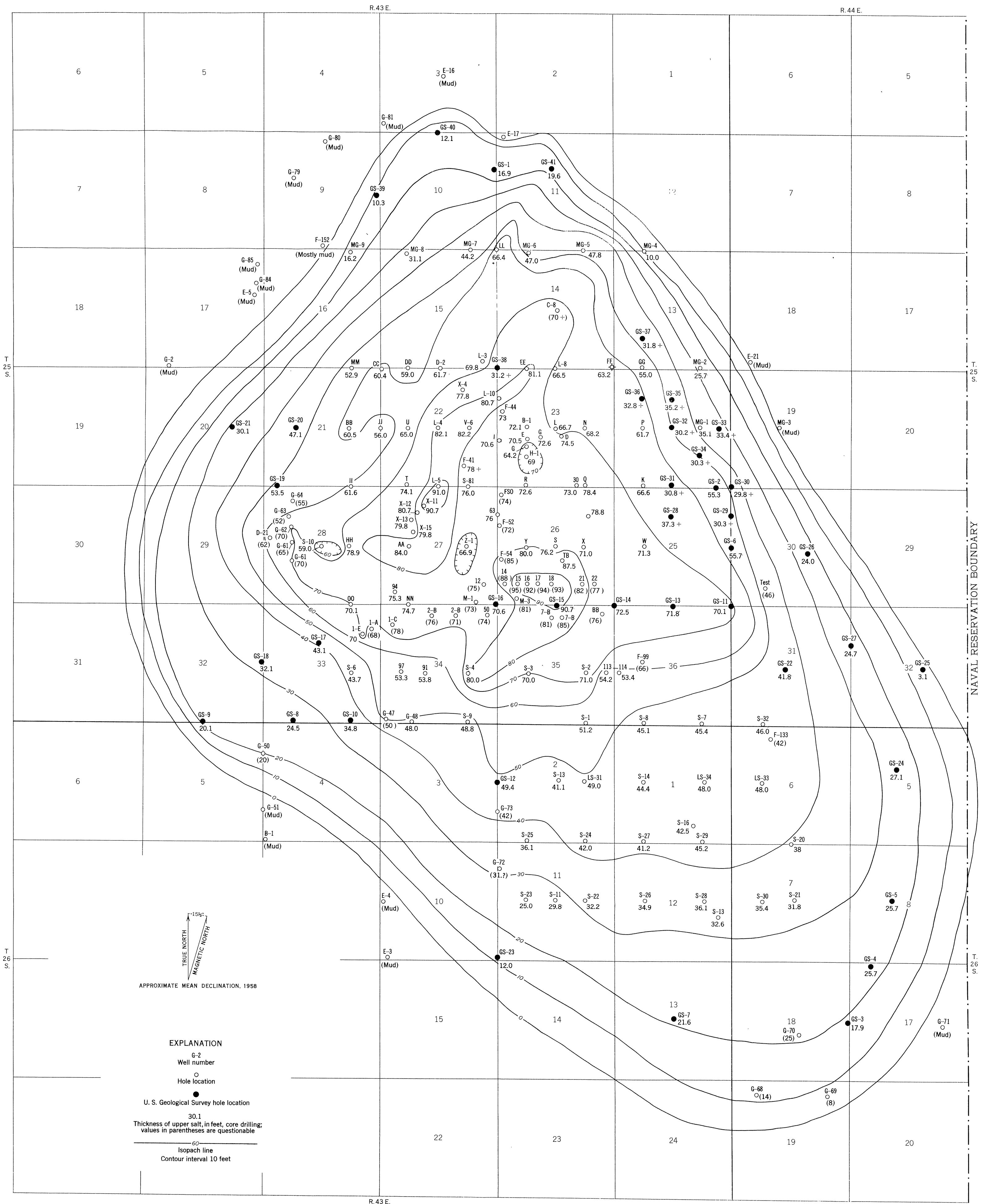
ISOPACH MAP OF UPPER SALT BODY, SEARLES LAKE, CALIFORNIA
