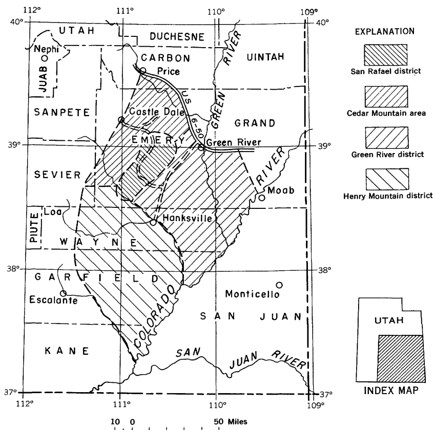
FIGURE 12.—Index map of part of Utah showing location of the San Rafael district and adjacent districts.
