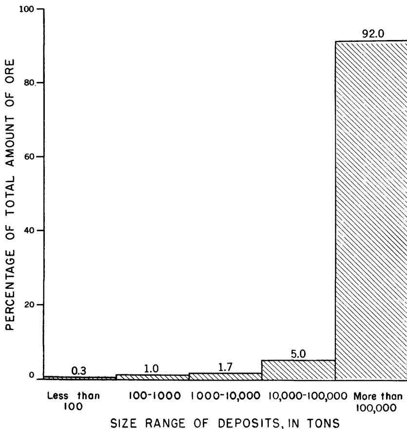
FIGURE 13.—Bar graph showing percentage of the total amount of ore (production through 1954 plus indicated and inferred reserves) in the San Rafael district that is contained in deposits of various size ranges.
