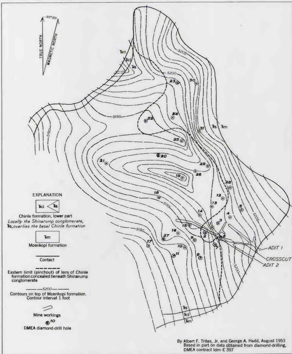
A. STRUCTURE CONTOUR MAP ON THE TOP OF THE MOENKOPI FORMATION
