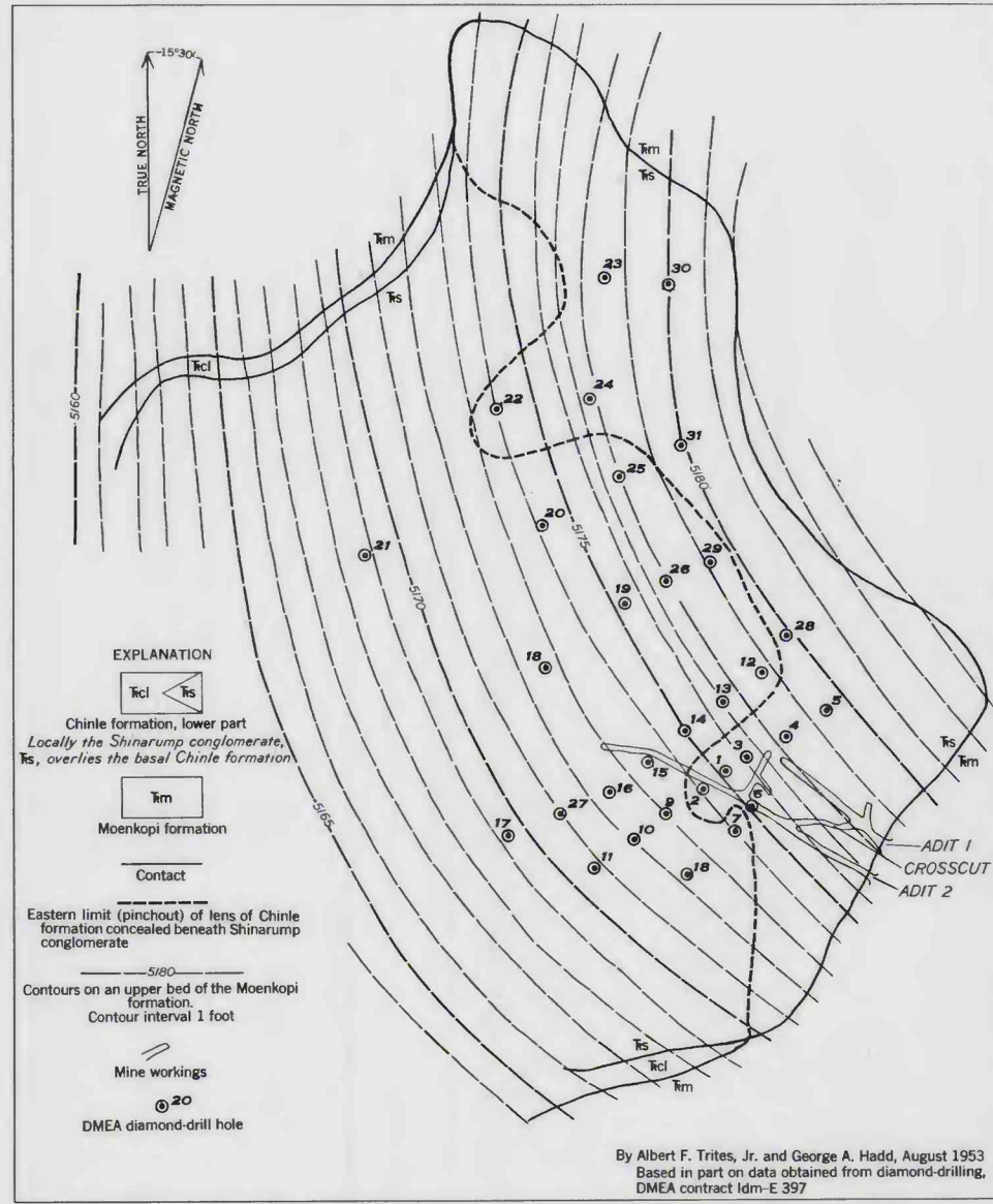
B. STRUCTURE CONTOUR MAP ON AN UPPER BED OF THE MOENKOPI FORMATION
