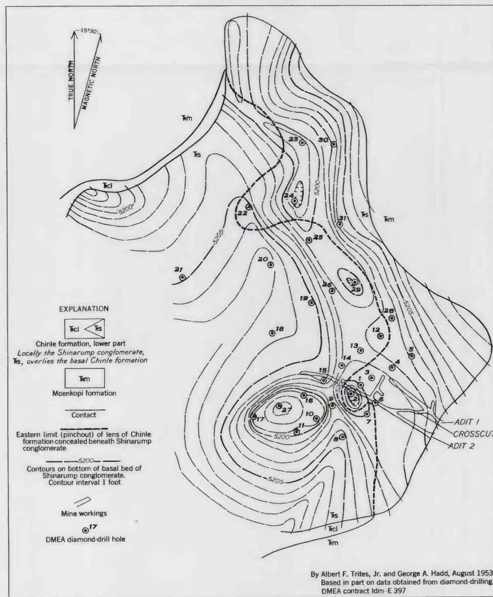
D. STRUCTURE CONTOUR MAP ON THE BOTTOM OF THE BASAL SANDSTONE OF THE SHINARUMP CONGLOMERATE
