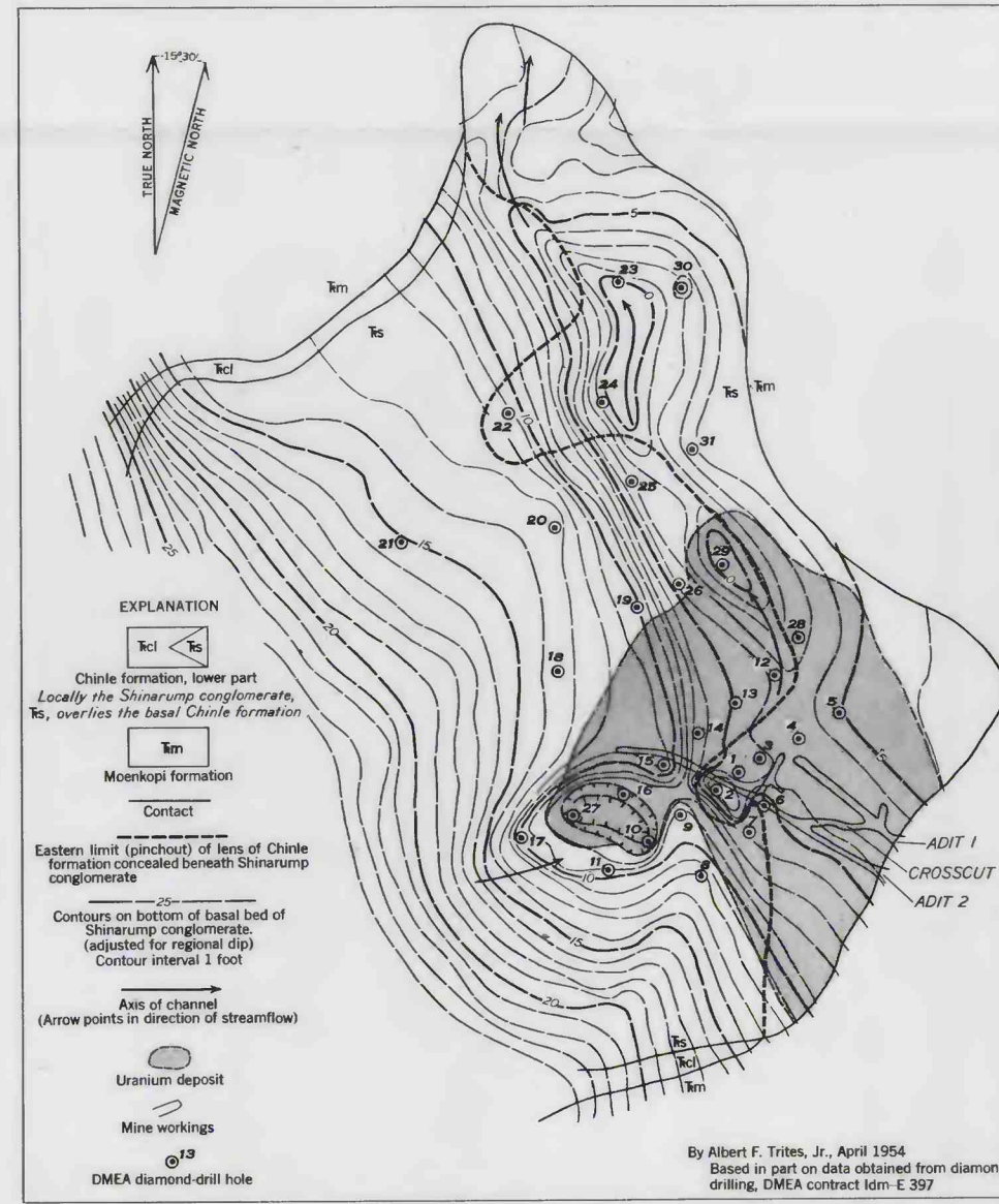
E. STRUCTURE CONTOUR MAP ON THE BOTTOM OF THE BASAL BED OF THE SHINARUMP CONGLOMERATE (ADJUSTED FOR REGIONAL DIP)
