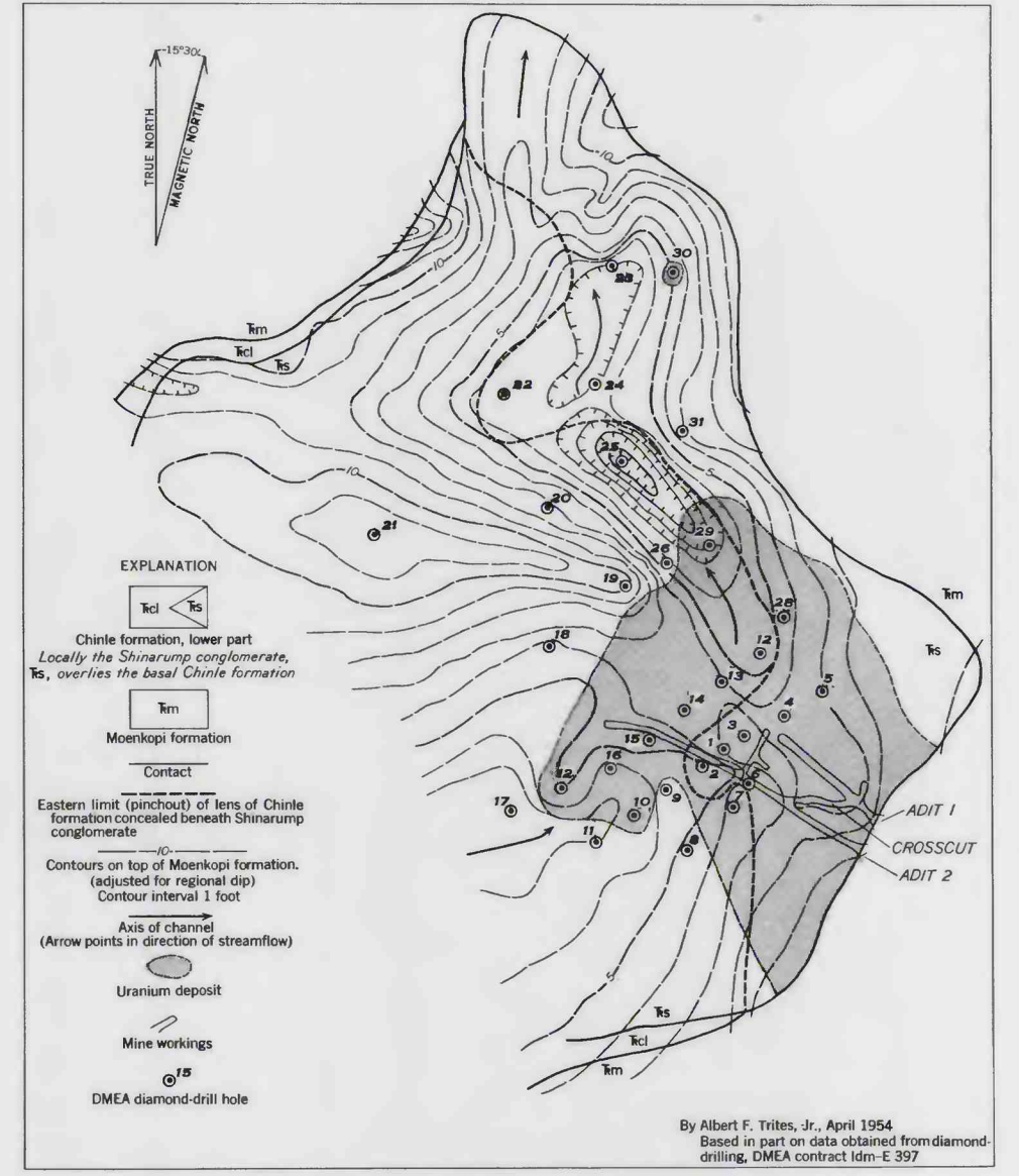
C. STRUCTURE CONTOUR MAP ON THE TOP OF THE MOENKOPI FORMATION (ADJUSTED FOR REGIONAL DIP)
