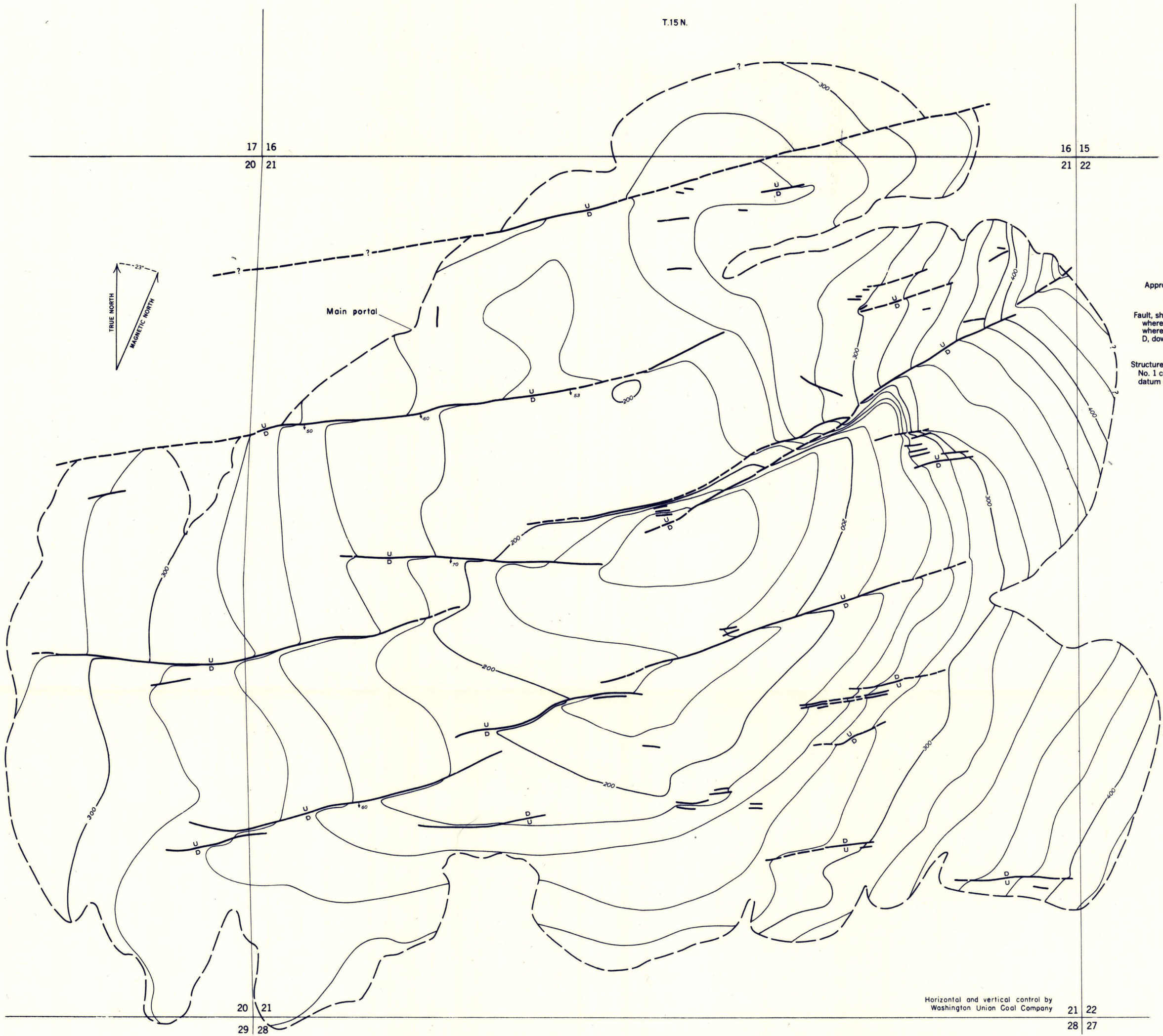
STRUCTURE-CONTOUR MAP OF TONO NO. 1 BED IN THE VICINITY OF TONO, WASHINGTON
