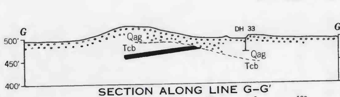
MAP AND SECTIONS OF COAL LOCALITY 3, LITTLE SUSITNA DISTRICT MATANUSKA COAL FIELD, ALASKA
