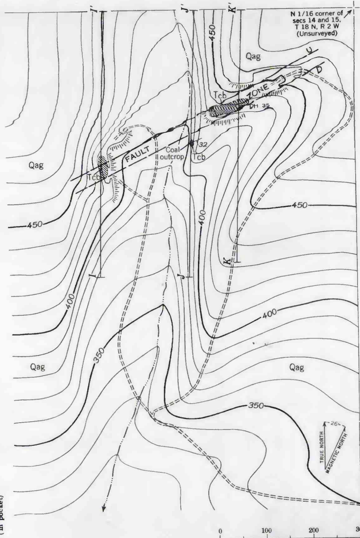
MAP AND SECTIONS OF COAL LOCALITY 4 LITTLE SUSITNA DISTRICT, MATANUSKA COAL FIELD, ALASKA
