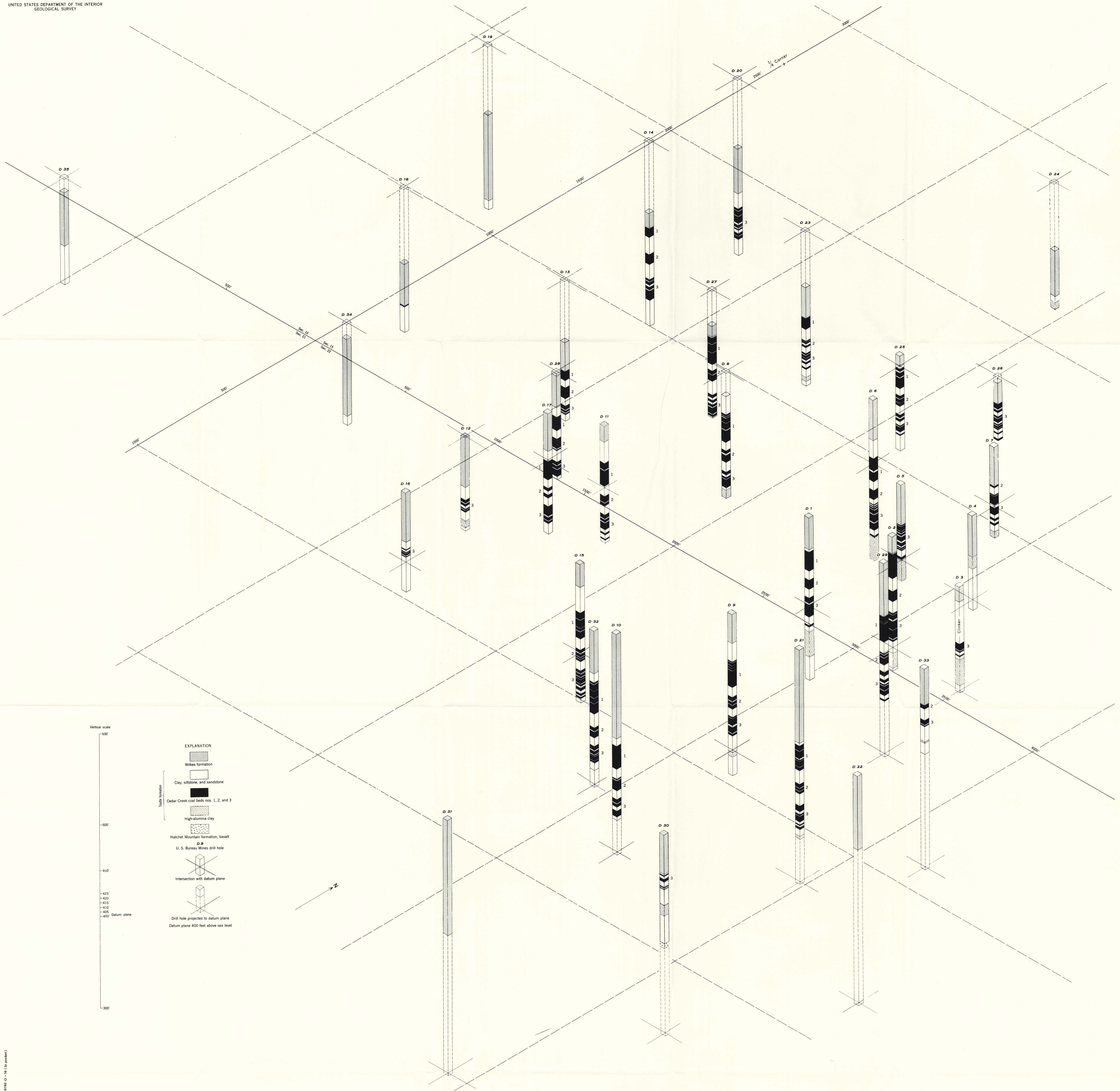
DIAGRAM SHOWING CORRELATIONS, RANGES IN THICKNESS, AND PRE-UPPER MIOCENE EROSION OF THE CEDAR CREEK NOS. 1, 2, AND 3 COAL BEDS IN SECS. 15, 16, 21, AND 22, T. 11 N., R. 1 E., LEWIS COUNTY, WASHINGTON
