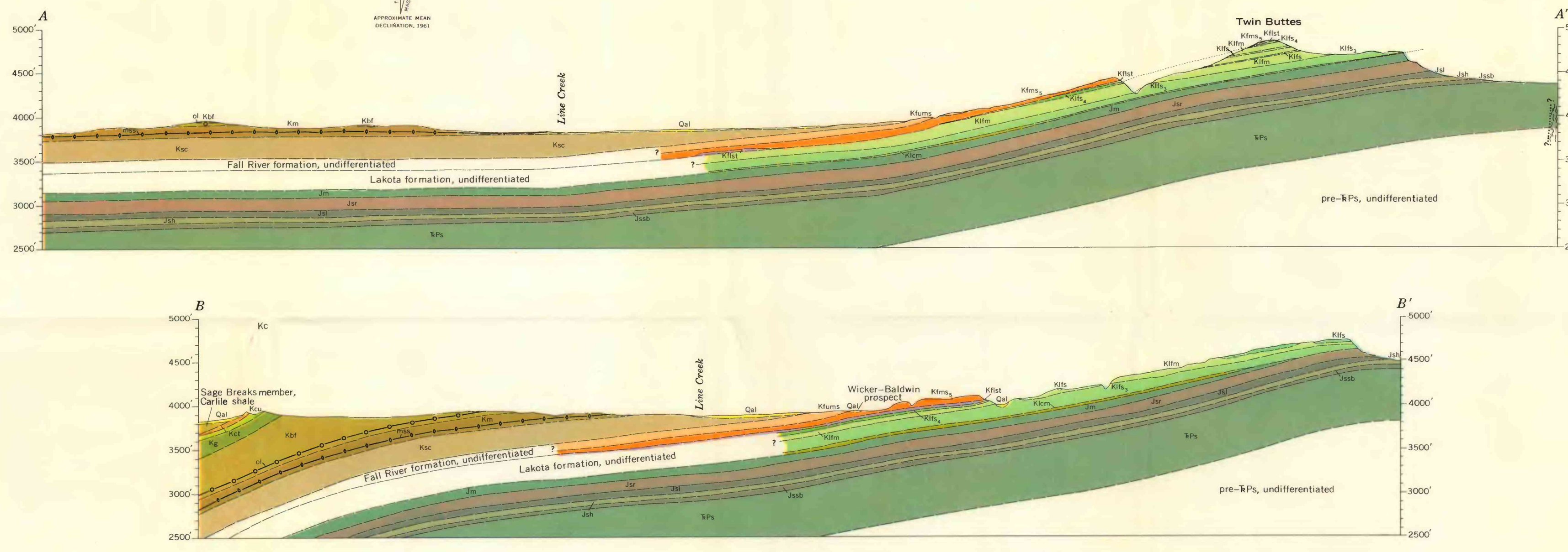
GEOLOGIC MAP AND SECTIONS OF THE DEWEY QUADRANGLE, WYOMING-SOUTH DAKOTA
