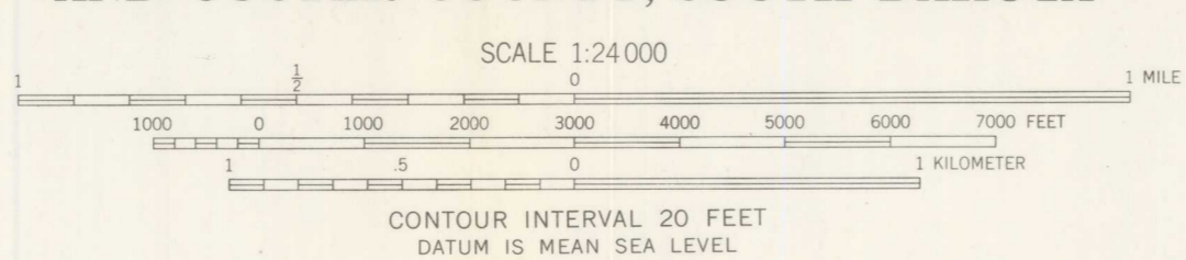
GEOLOGIC MAP AND SECTIONS OF THE CLIFTON QUADRANGLE, WESTON COUNTY, WYOMING AND CUSTER COUNTY, SOUTH DAKOTA
