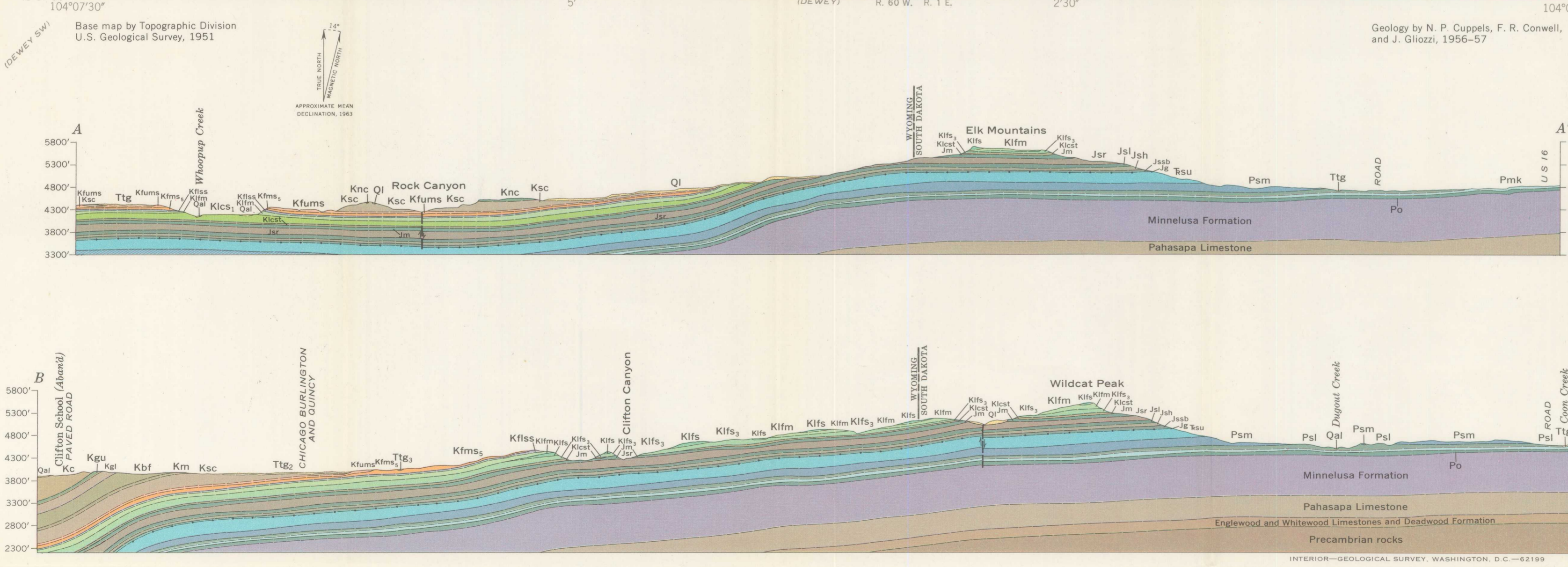
GEOLOGIC MAP AND SECTIONS OF THE CLIFTON QUADRANGLE, WESTON COUNTY, WYOMING AND CUSTER COUNTY, SOUTH DAKOTA
