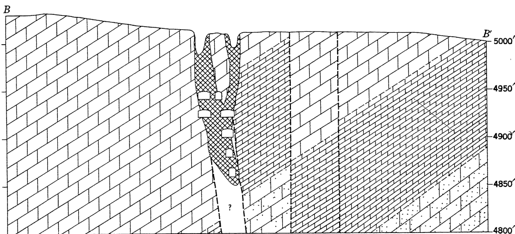
GEOLOGIC SECTIONS OF THE LARGE PIPE ON THE BELL HILL PROPERTY
