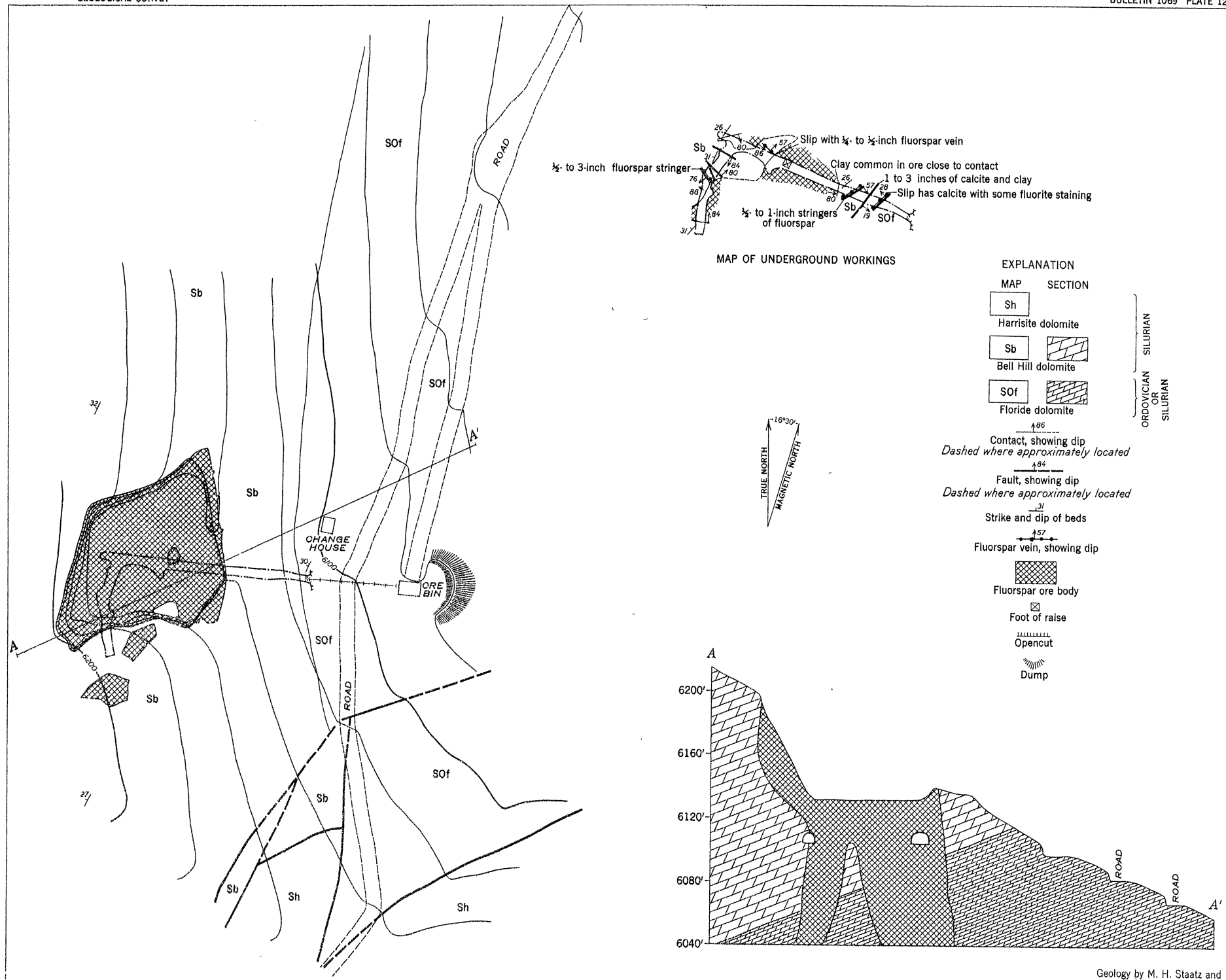
GEOLOGIC MAP AND SECTION OF THE EAST PIT OF THE FLUORINE QUEEN MINE, THOMAS RANGE, JUAB COUNTY, UTAH
