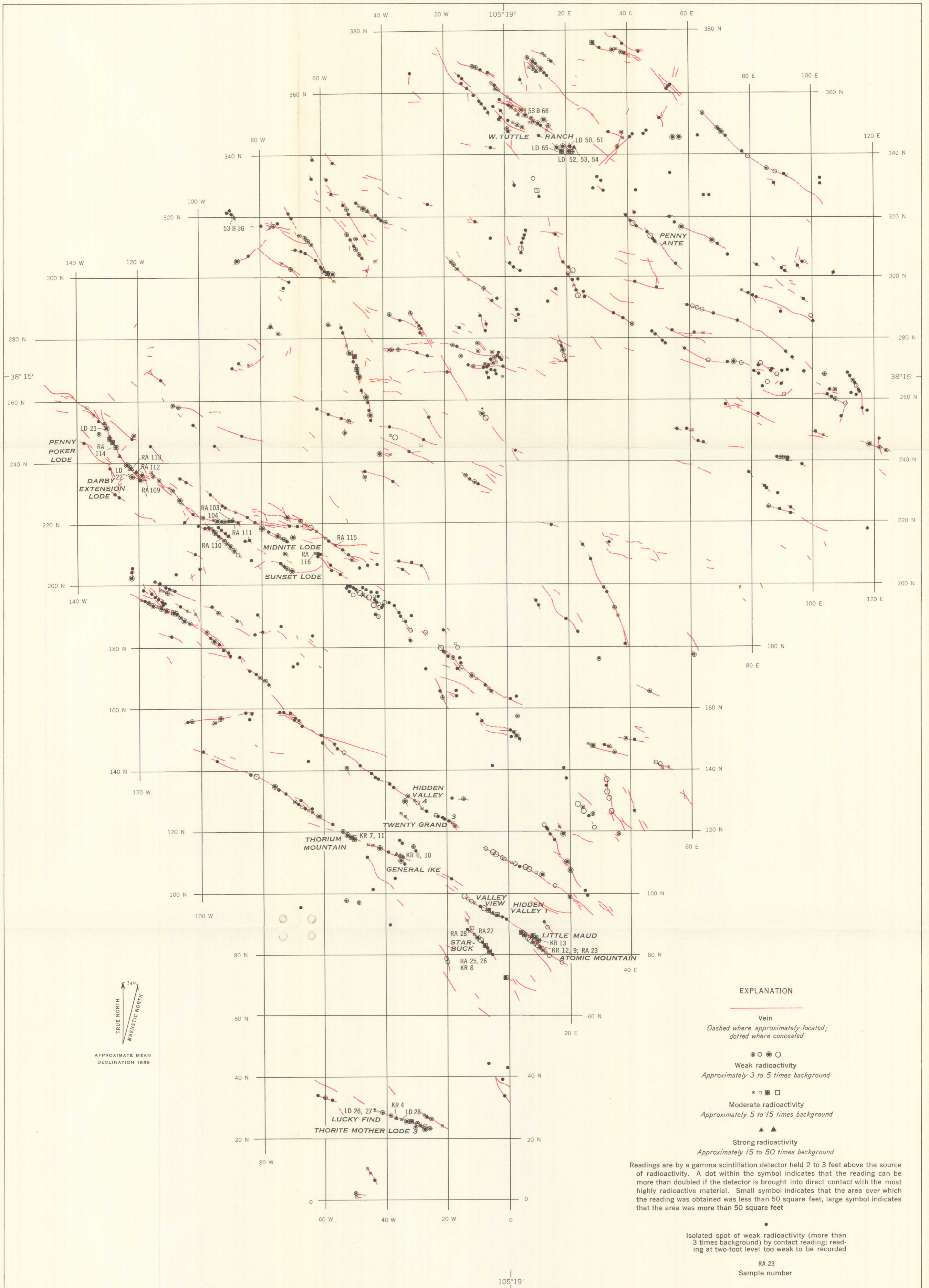
INDEX MAP SHOWING LOCALITIES OF RADIOACTIVE MATERIAL, MCKINLEY MOUNTAIN AREA, WET MOUNTAINS, COLORADO
