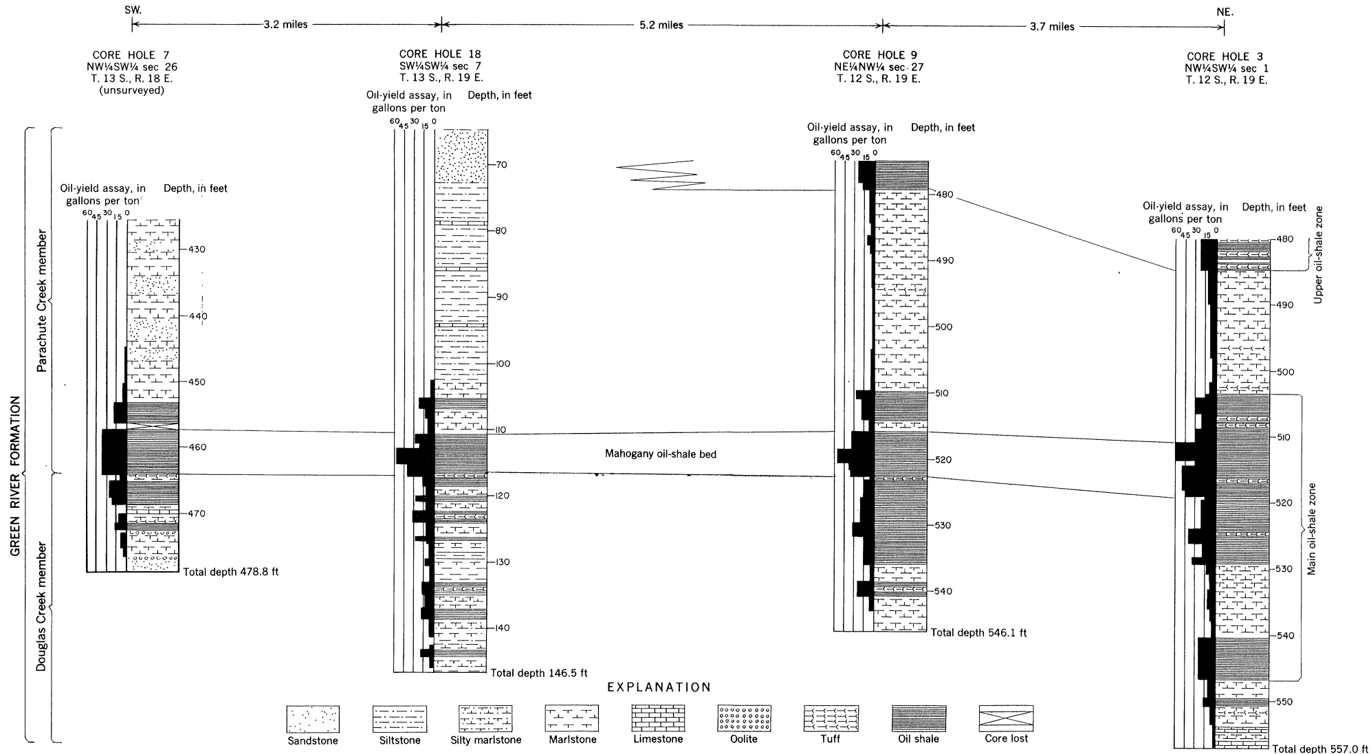
LINE OF GRAPHIC SECTIONS SHOWING DECREASE IN SHALE OIL CONTENT IN A SOUTHWESTERLY DIRECTION, NAVAL OIL-SHALE RESERVE NO. 2, Uintah County, Utah
