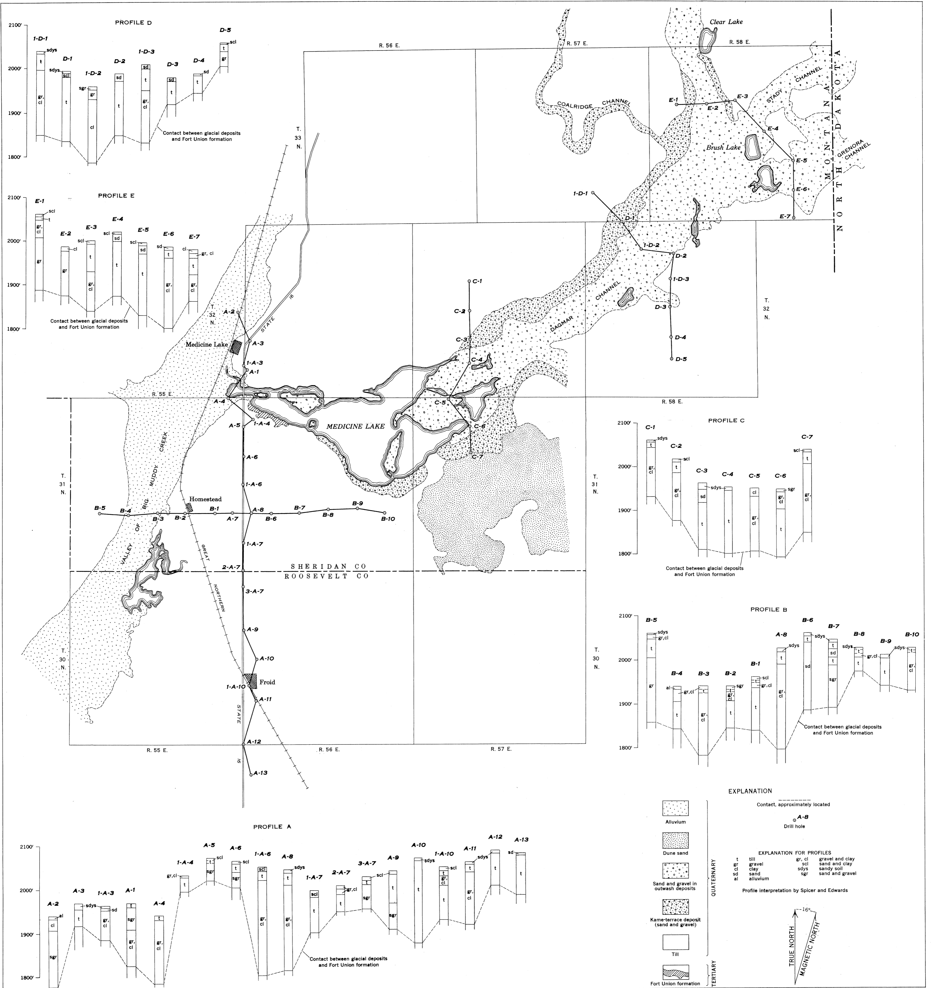
GENERALIZED GEOLOGIC MAP OF AREA NEAR MEDICINE LAKE, MONTANA, WITH GEOLOGIC INTERPRETATION OF FIVE RESISTIVITY PROFILES
