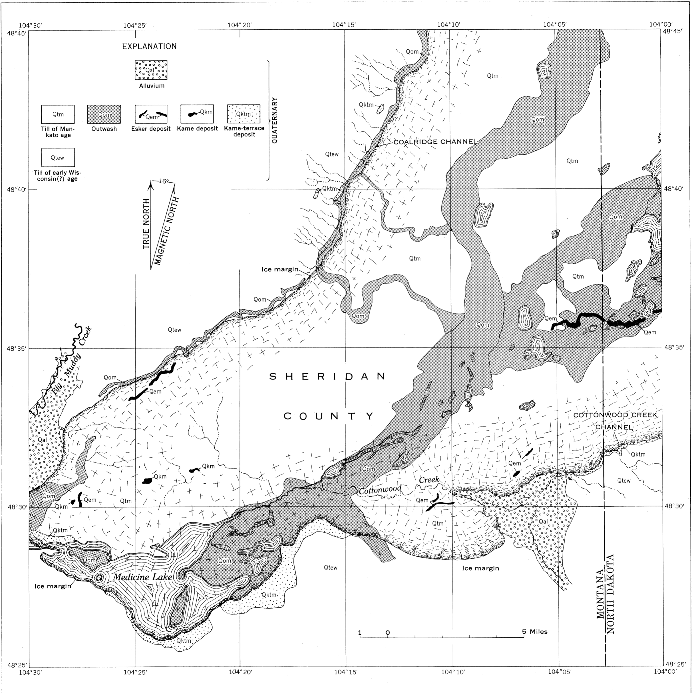
SKETCH MAP SHOWING PROBABLE EXTENT OF LOBE OF MANKATO ICE DOWN SAG FORMED BY DAGMAR CHANNEL, SHERIDAN COUNTY, MONTANA
