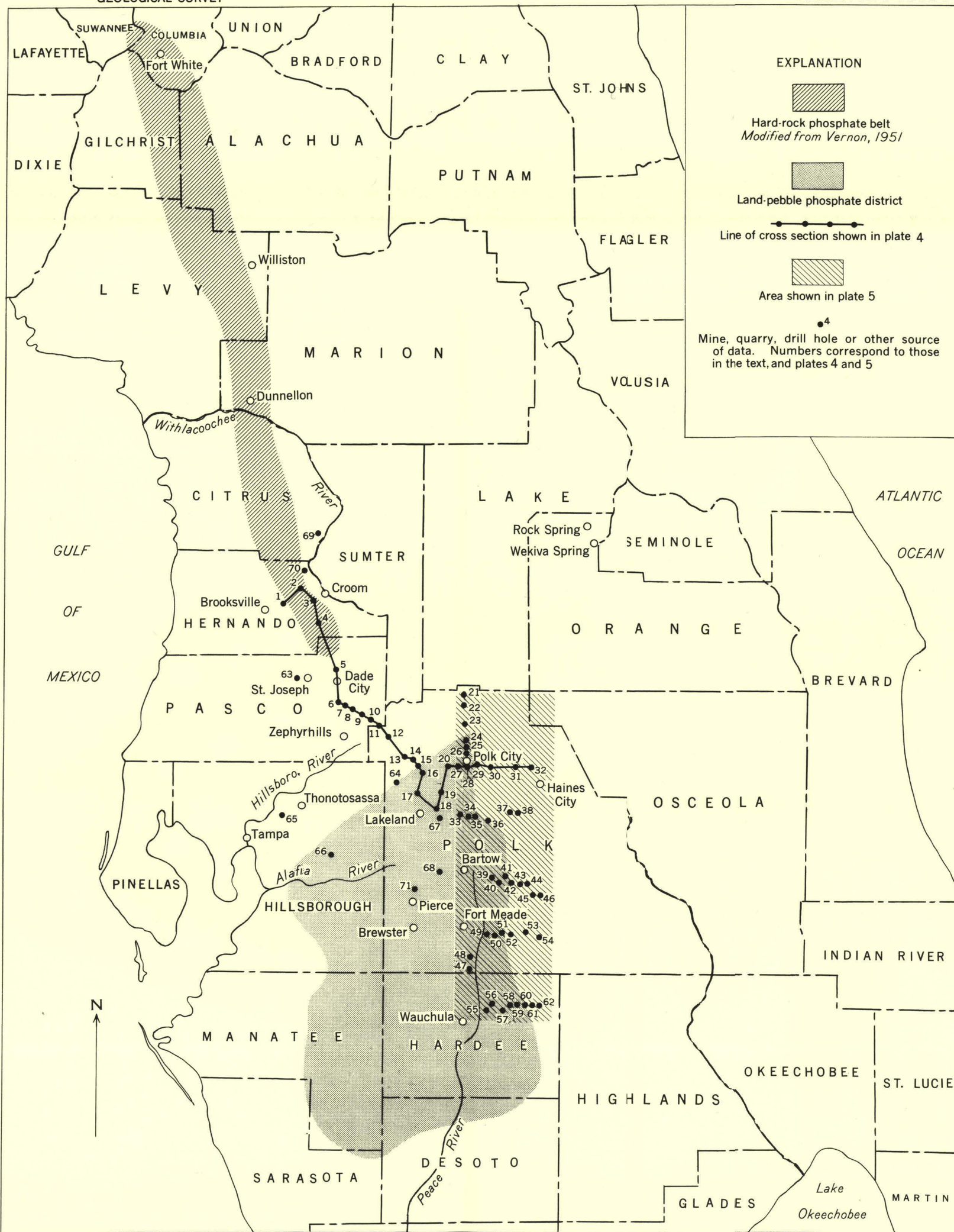
INDEX MAP OF CENTRAL FLORIDA SHOWING LOCATION OF SOURCES OF DATA
