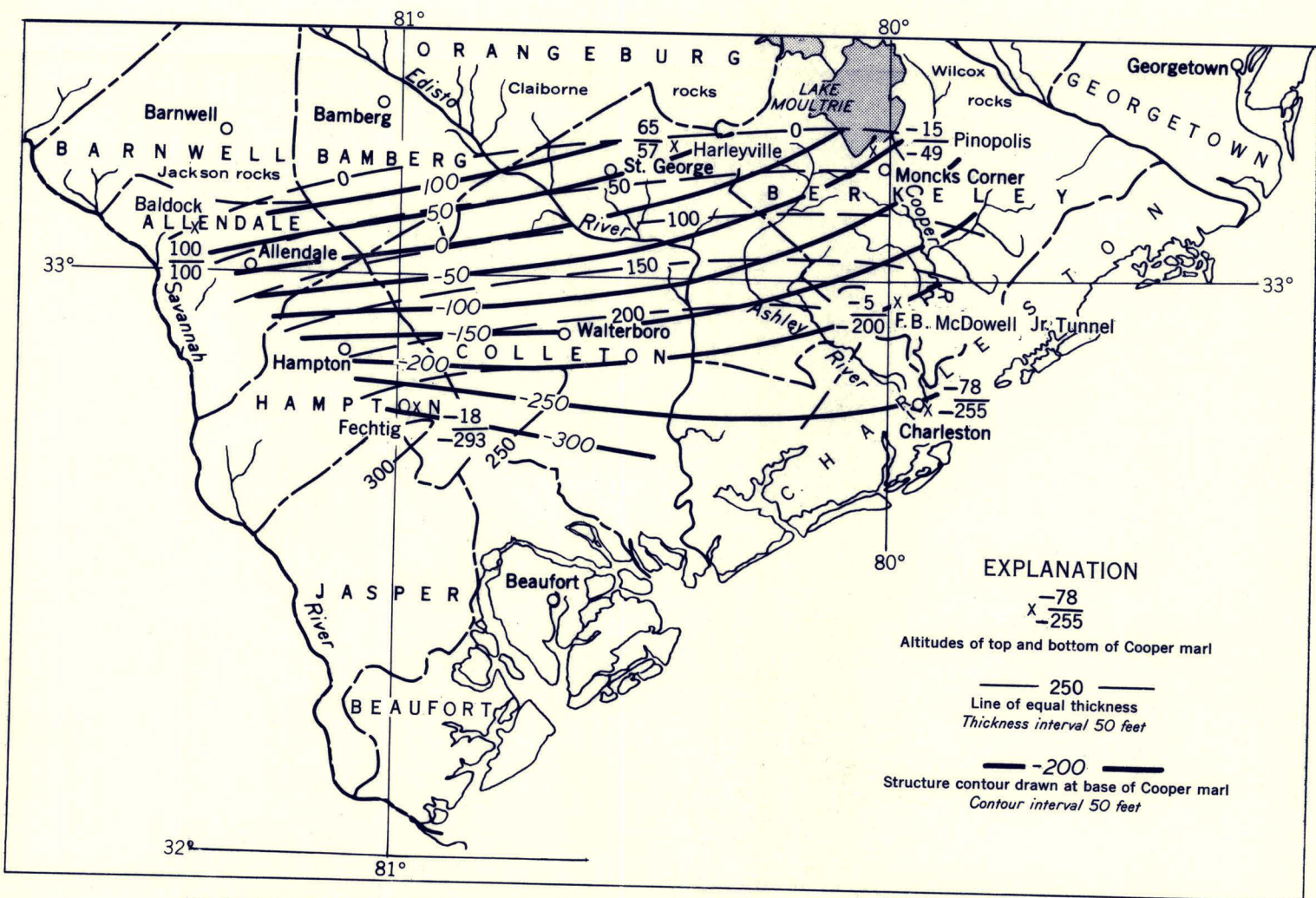
DIAGRAM SHOWING THE STRATIGRAPHY, STRUCTURAL ATTITUDE, AND THICKNESS OF THE COOPER MARL IN SOUTH CAROLINA
