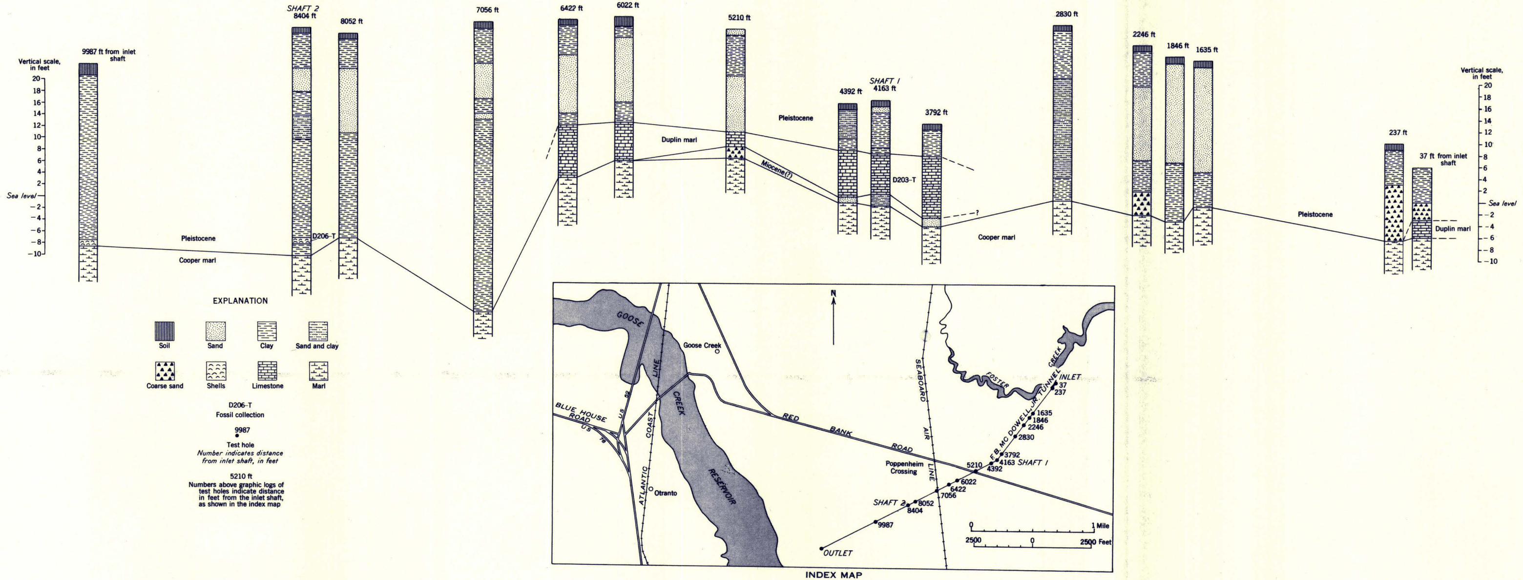
CORRELATION OF BEDS FOUND IN HOLES DRILLED ALONG THE LINE OF THE F. B. MCDOWELL, JR., TUNNEL, FOSTER CREEK TO GOOSE CREEK, SOUTH CAROLINA
