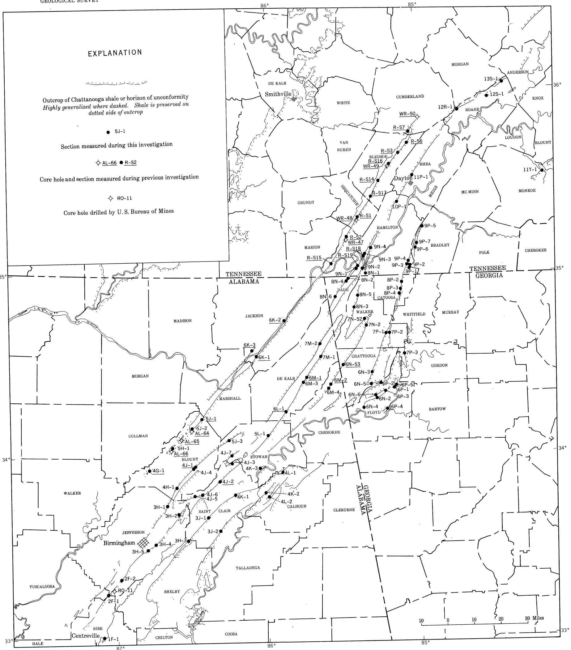
CHATTANOOGA SHALE LOCALITIES IN NORTHEASTERN ALABAMA, NORTHWESTERN GEORGIA, AND EASTERN TENNESSEE
