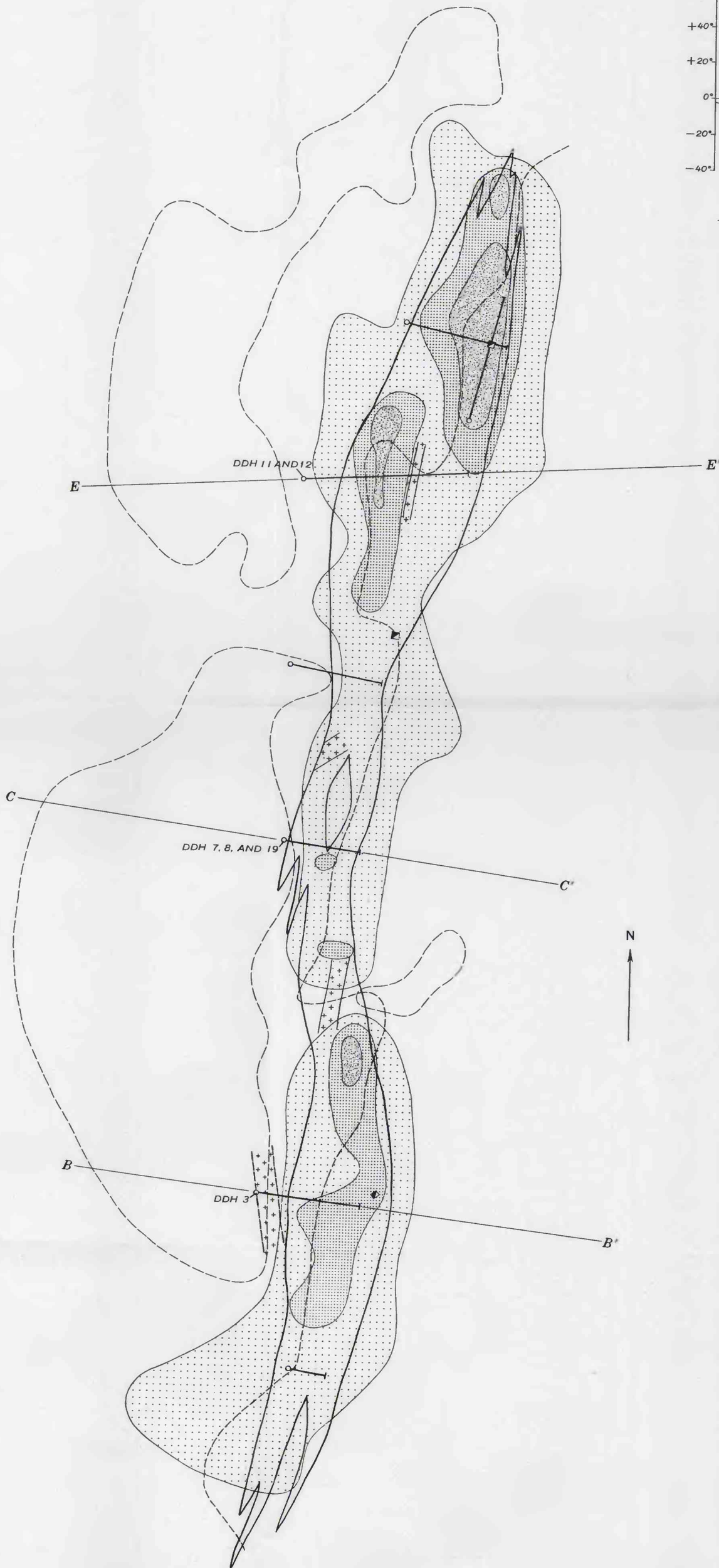
MAGNETIC MAP AND PROFILES, POOR MAN IRON DEPOSIT
