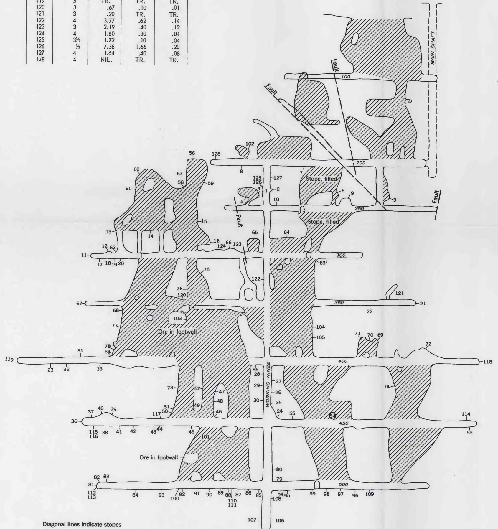
SECTION ON VEIN OF RUSH AND BROWN MINE, SHOWING LOCATIONS OF SAMPLES
