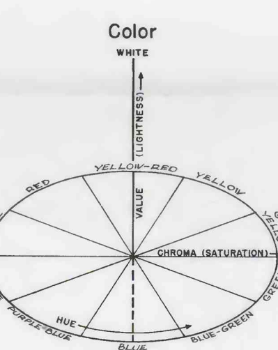
Color solid dimensions of the Munsell system (Goddard and others, 1948)
