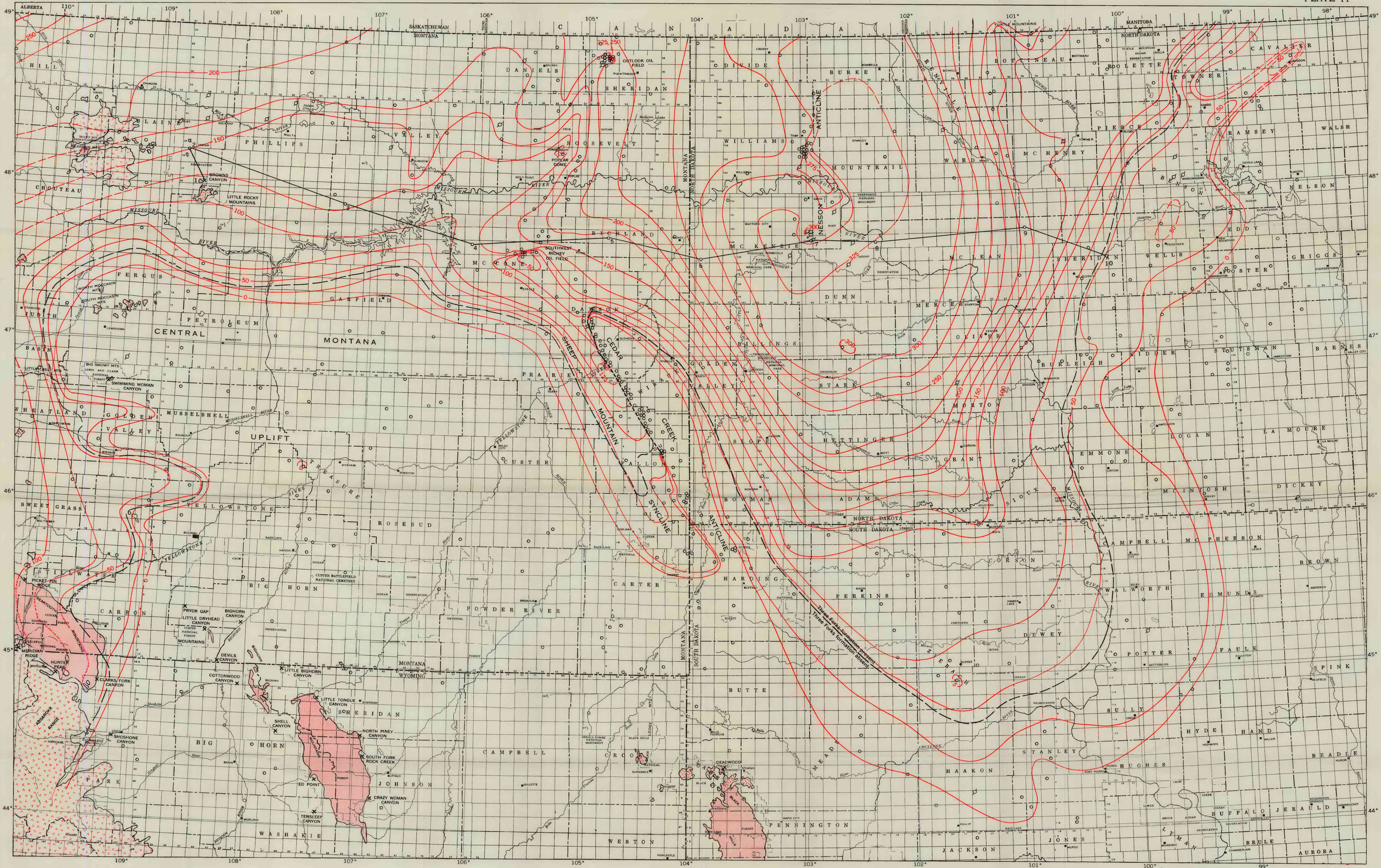
ISOPACH MAP OF BIRDBEAR AND THREE FORKS FORMATIONS IN WILLISTON BASIN AND IN CENTRAL MONTANA AND NORTH-CENTRAL WYOMING
