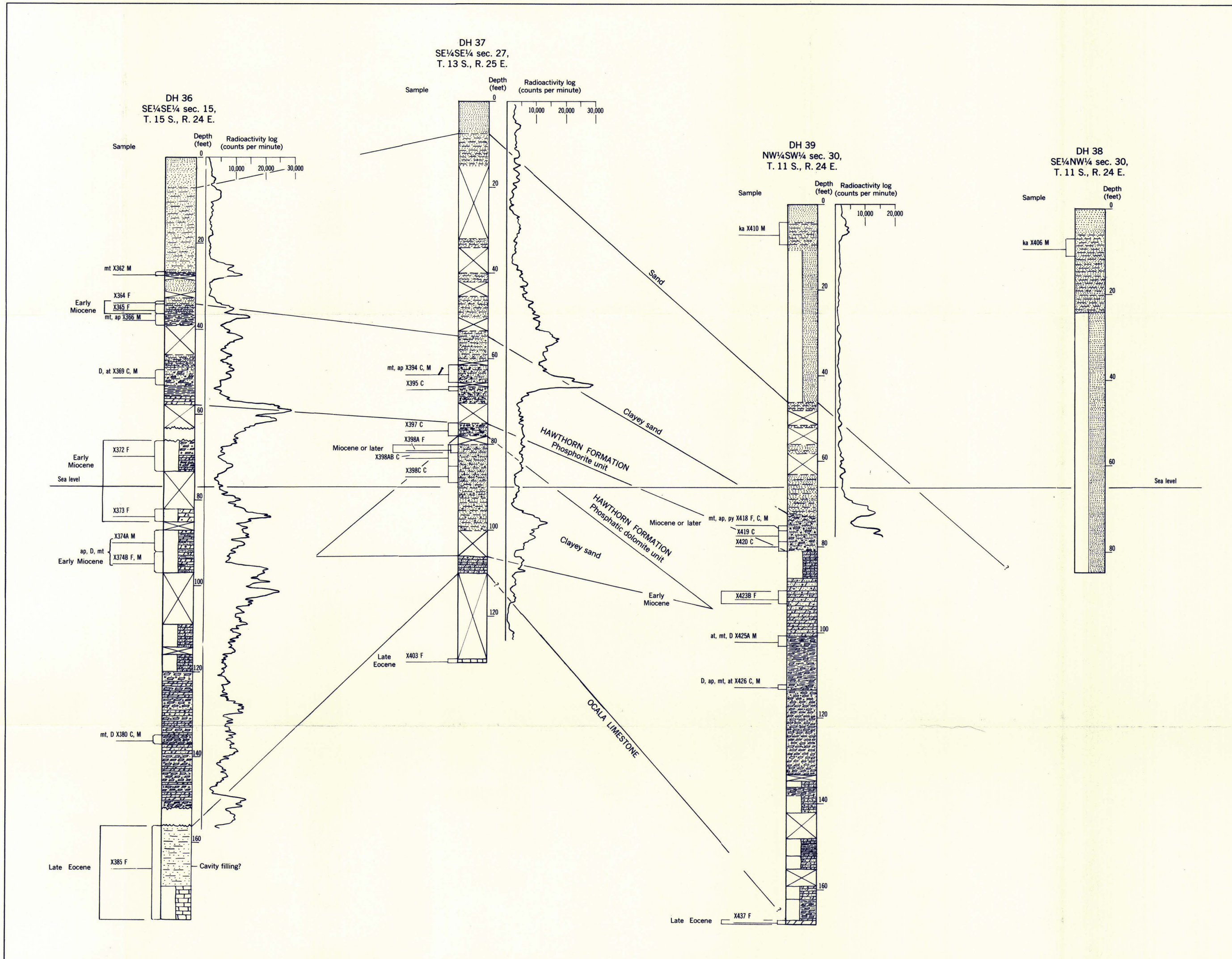
GRAPHIC LOGS OF CORES FROM DRILL HOLES 36 TO 39 NORTHERN PENINSULAR FLORIDA
