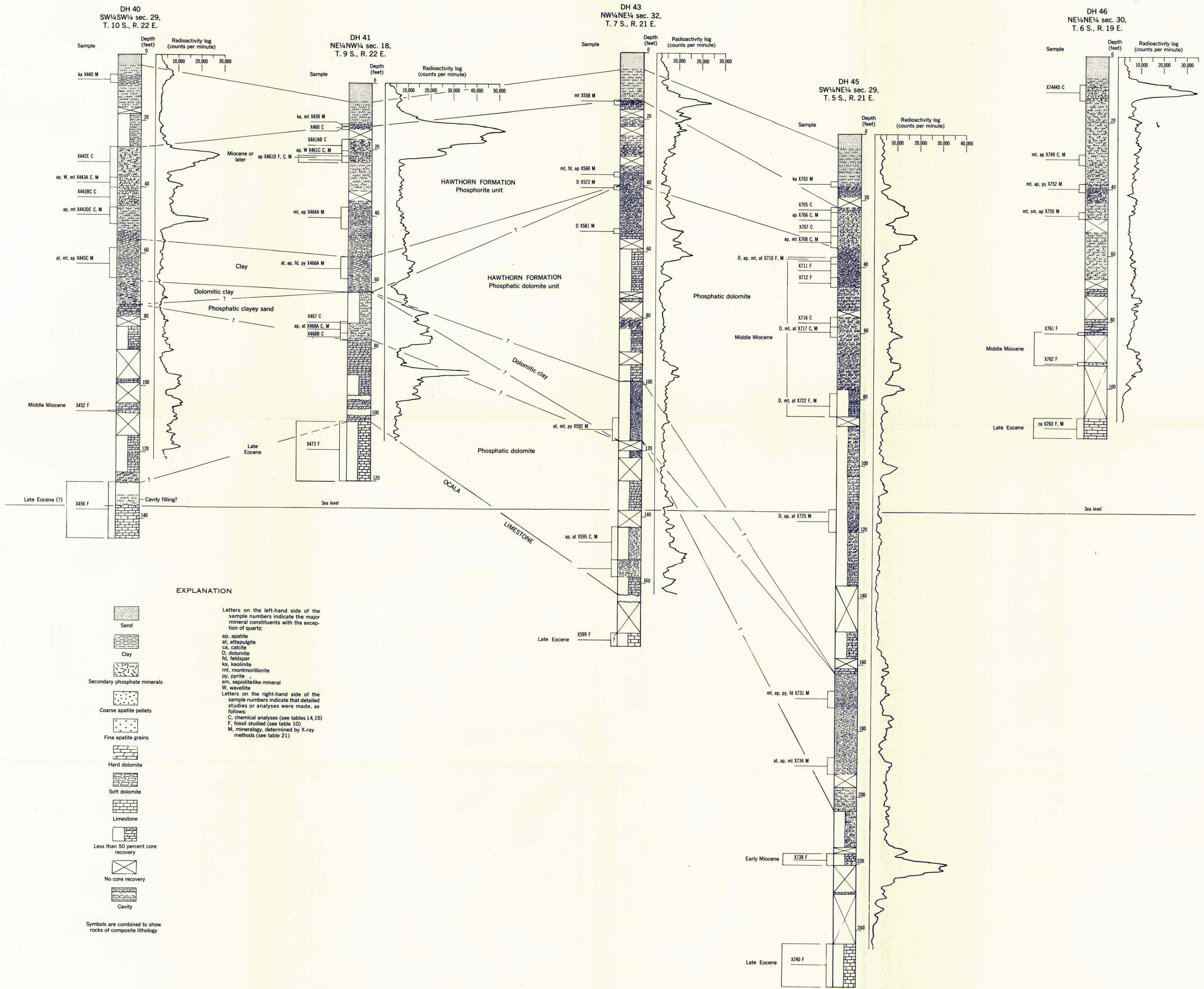
GRAPHIC LOGS OF CORES FROM DRILL HOLES 40, 41, 43, 45, AND 46 NORTHERN PENINSULAR FLORIDA
