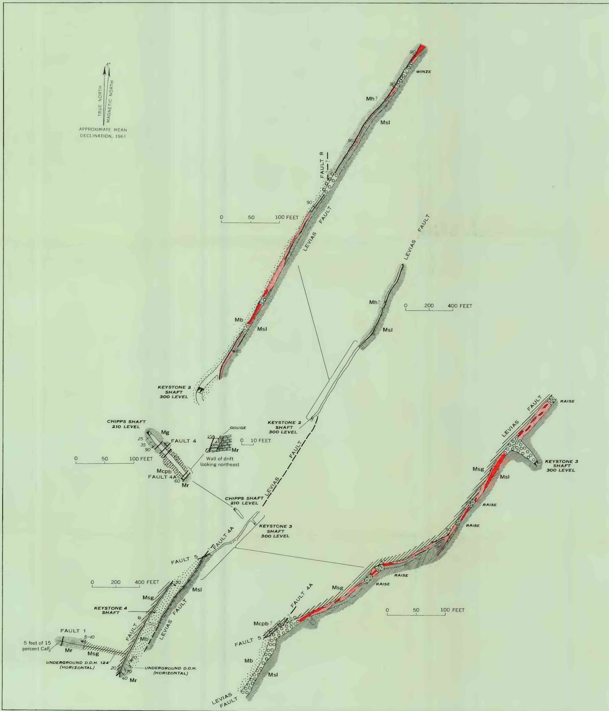
UNDERGROUND GEOLOGIC MAP OF PART OF THE KEYSTONE MINE AND THE CHIPPS SHAFT KEYSTONE AREA, CRITTENDEN COUNTY, KENTUCKY
