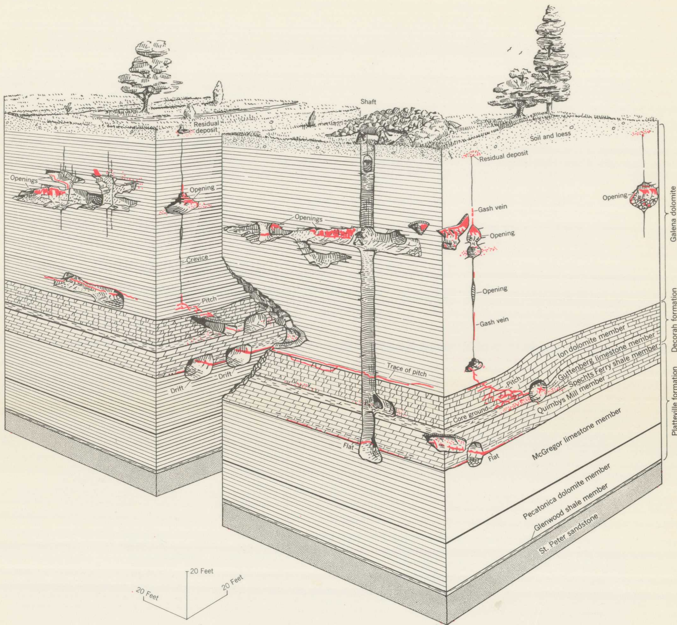
DIAGRAM SHOWING THE RELATION BETWEEN RESIDUAL DEPOSITS, JOINT-CONTROLLED DEPOSITS, AND PITCH-AND-FLAT DEPOSITS IN THE MINERAL POINT AREA, WISCONSIN
