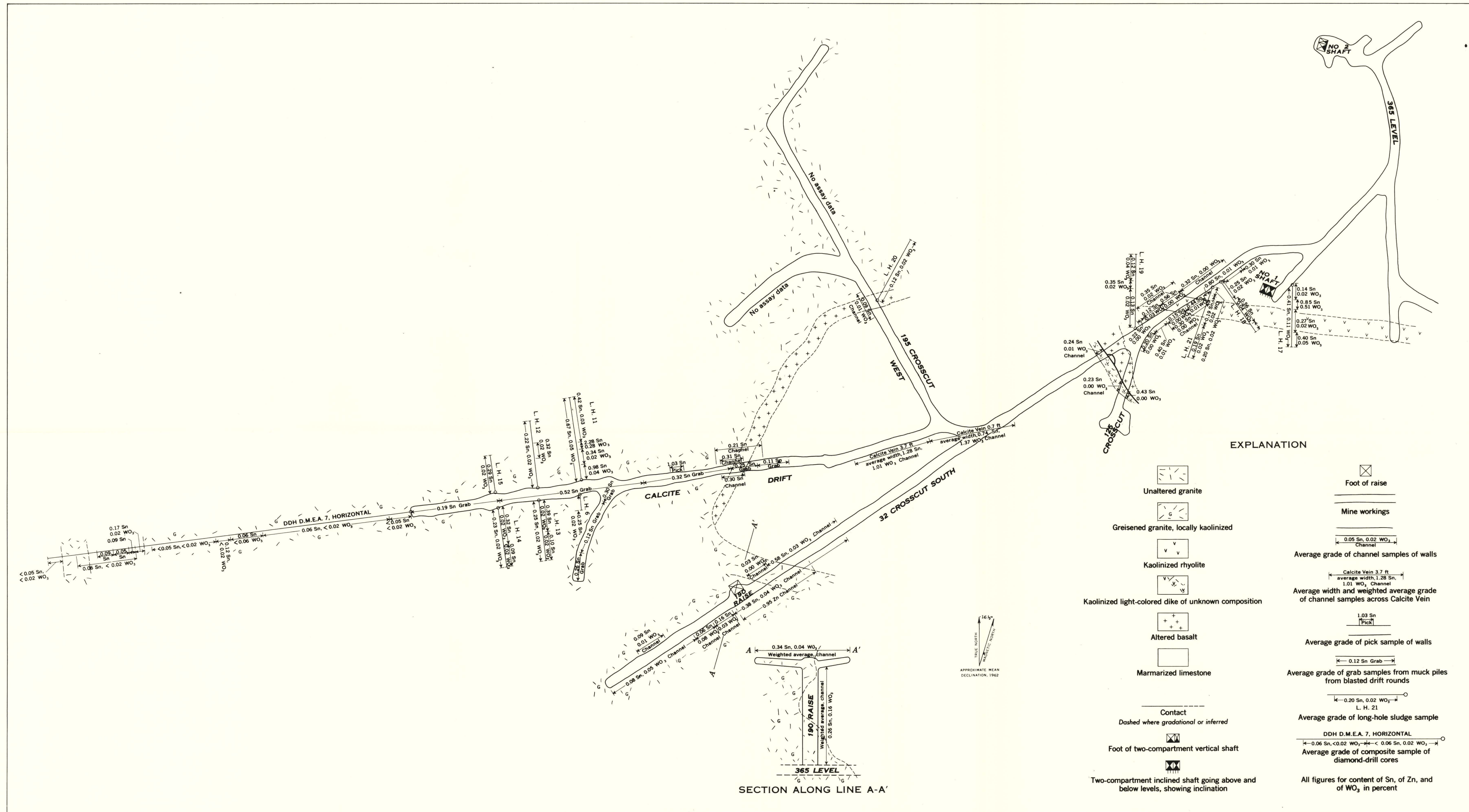
ASSAY MAP OF PART OF 365 LEVEL, LOST RIVER MINE, ALASKA
