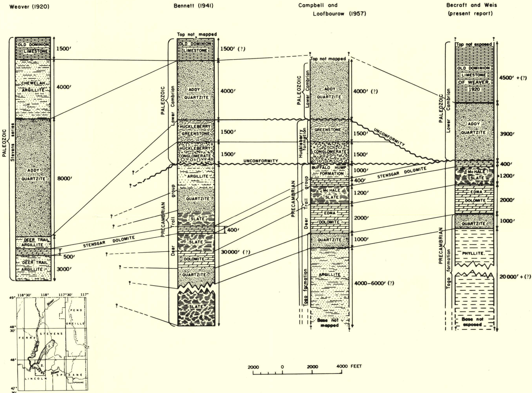
CORRELATION CHART SHOWING STRATIGRAPHIC SECTIONS OF THE MAGNESITE BELT SOUTHERN STEVENS COUNTY, WASHINGTON, AS MAPPED BY DIFFERENT WORKERS
