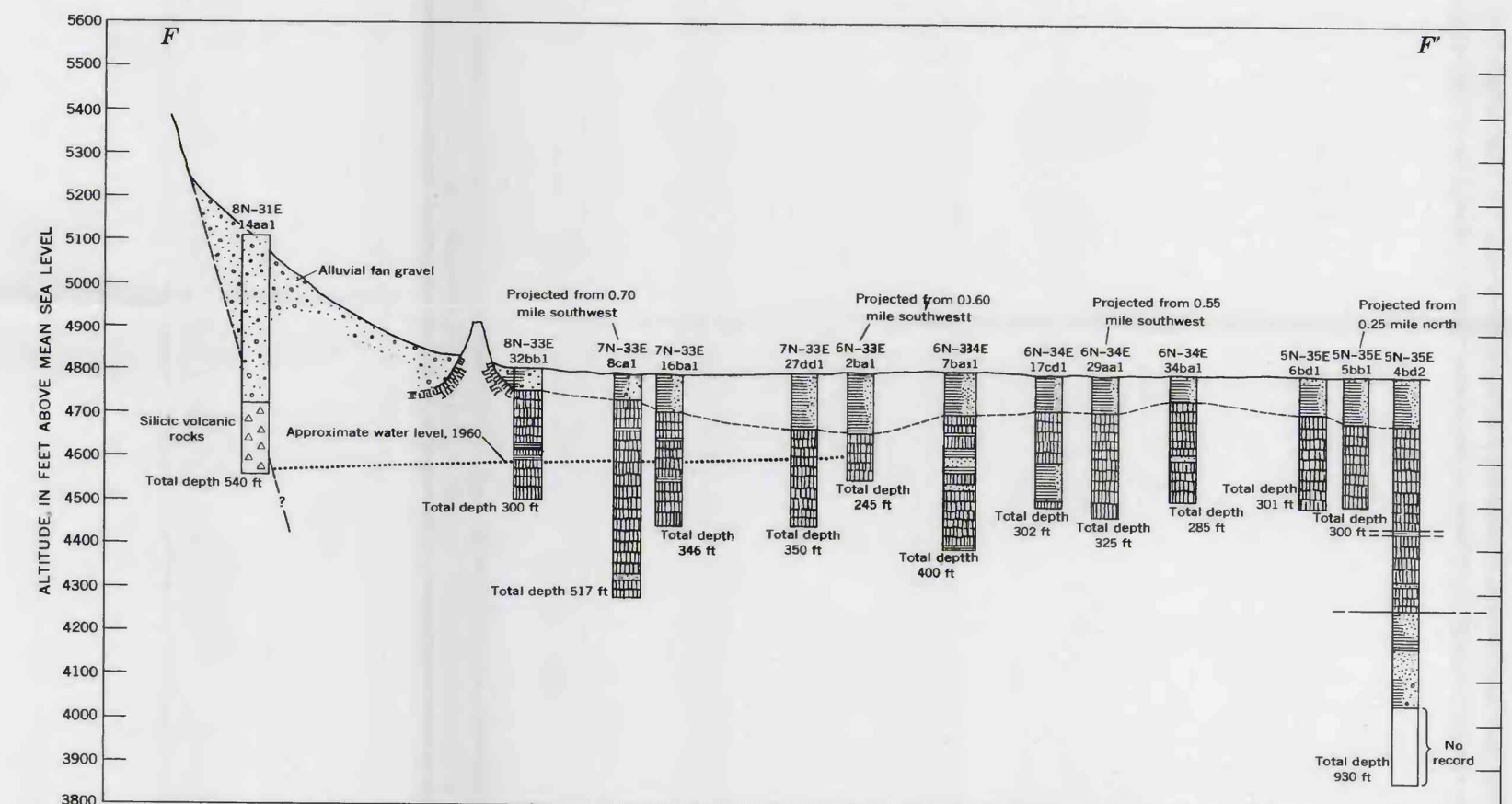
GEOLOGIC SECTIONS A-A' TO F-F', NATIONAL REACTOR TESTING STATION, IDAHO
