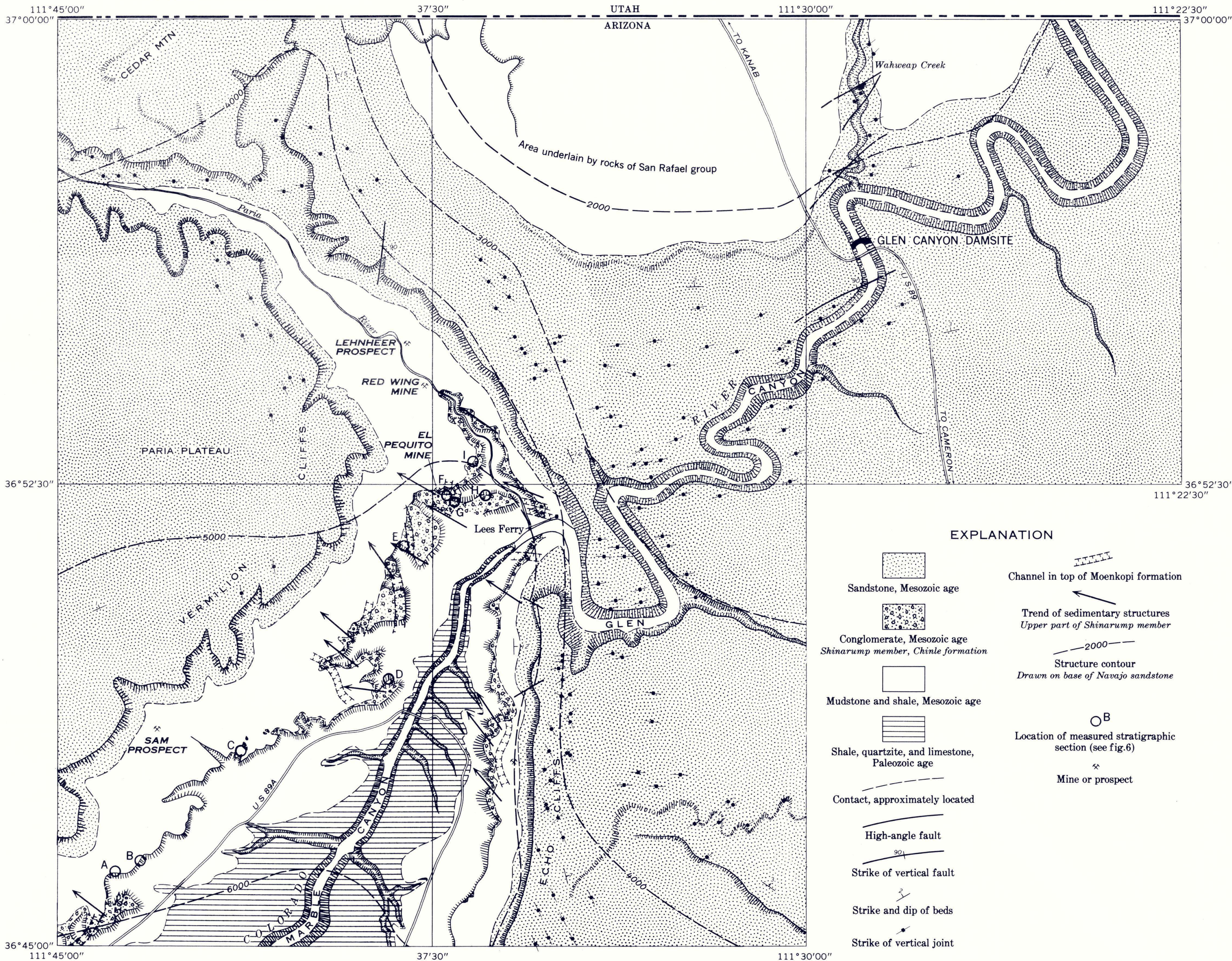
GENERALIZED GEOLOGIC MAP OF THE LEES FERRY AREA, COCONINO COUNTY, ARIZONA
