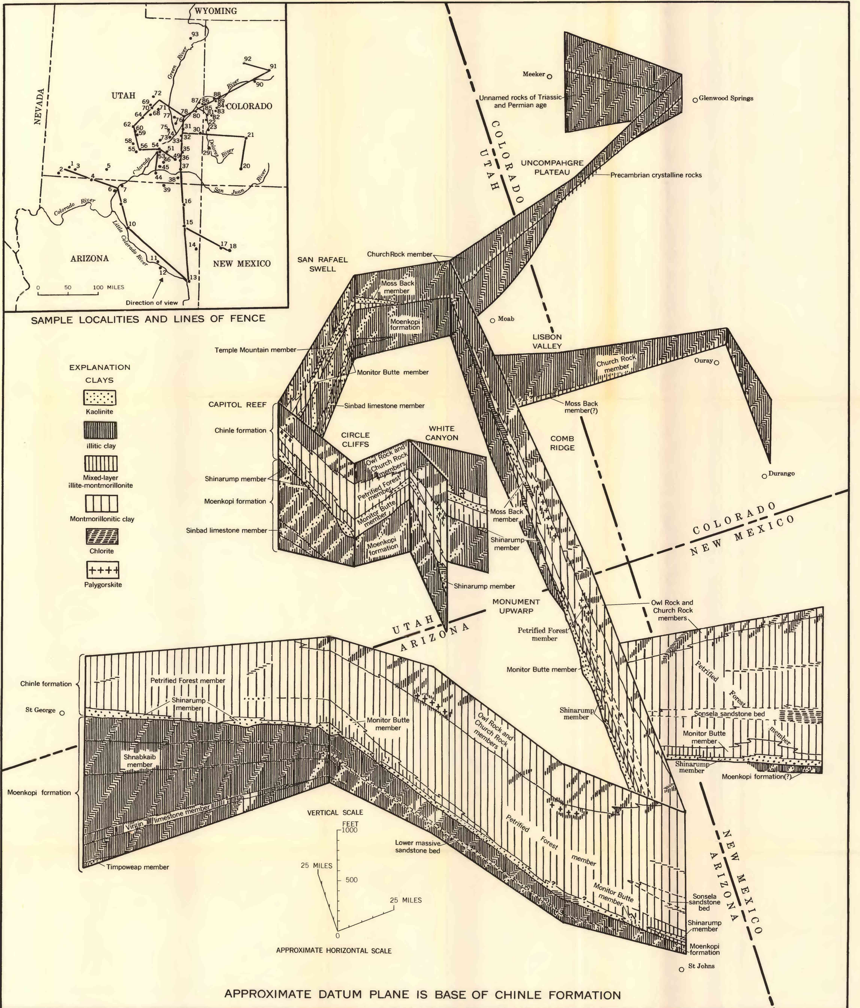
FENCE DIAGRAM SHOWING COMMON CLAYS IN THE TRIASSIC ROCKS OF THE COLORADO PLATEAU
