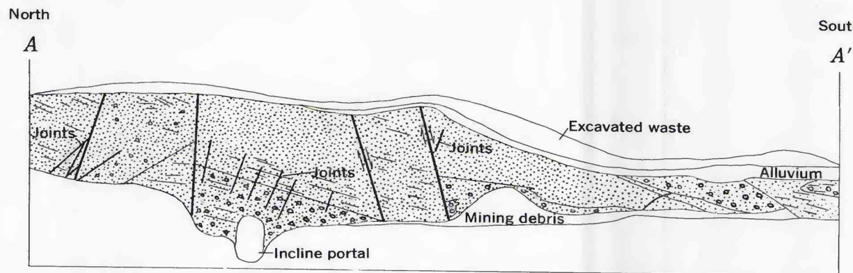
SECTION A-A' ALONG EAST FACE OF CUT
