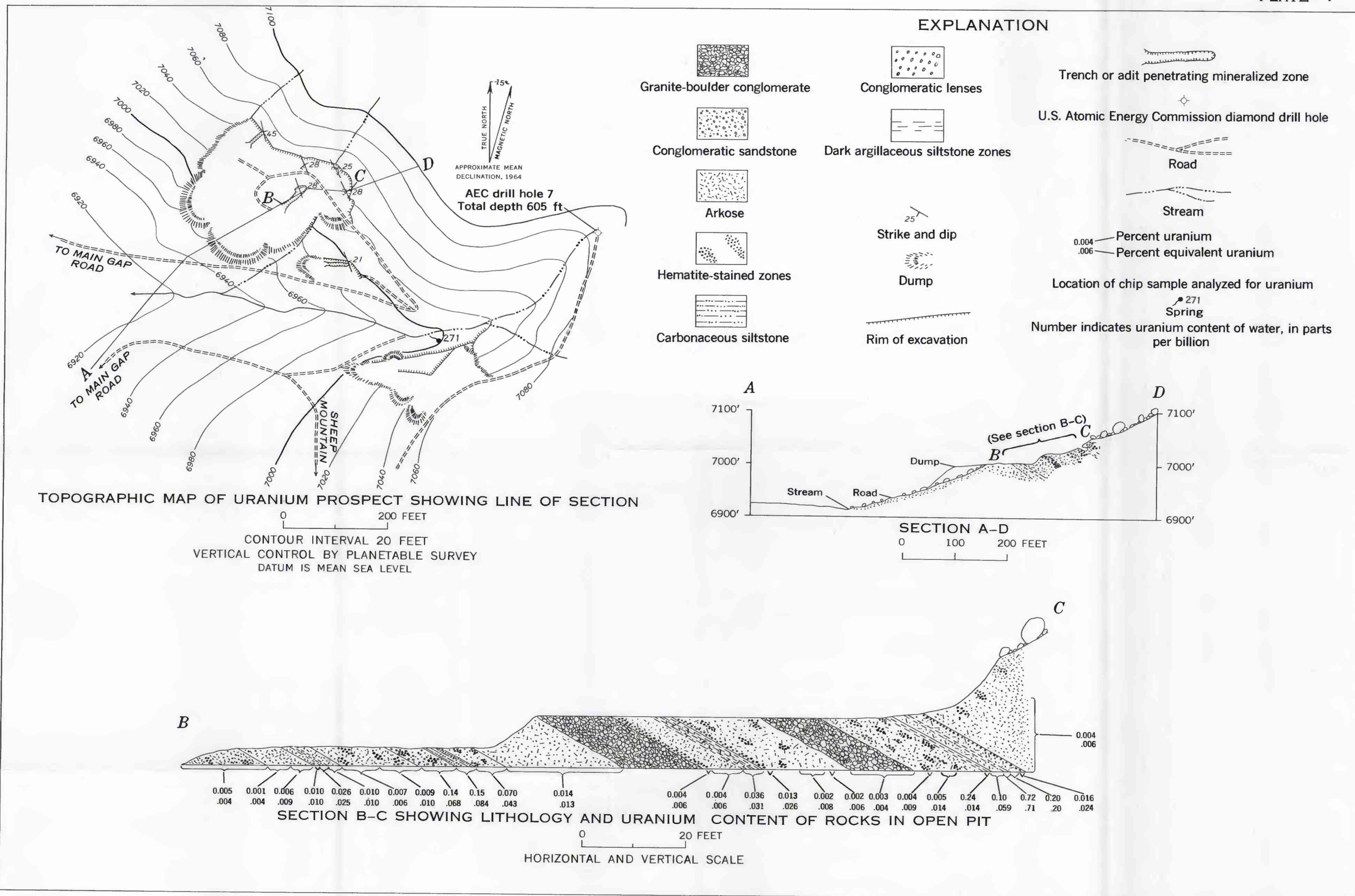
MAP AND GEOLOGIC SECTION OF PROSPECT PIT IN MEMBER A OF THE BATTLE SPRING FORMATION SUNDOG CLAIMS, SW \frac{1}{4} NW \frac{1}{4} SEC. 28, T. 28 N., R. 92 W., CROOKS GAP AREA, FREMONT COUNTY, WYOMING
