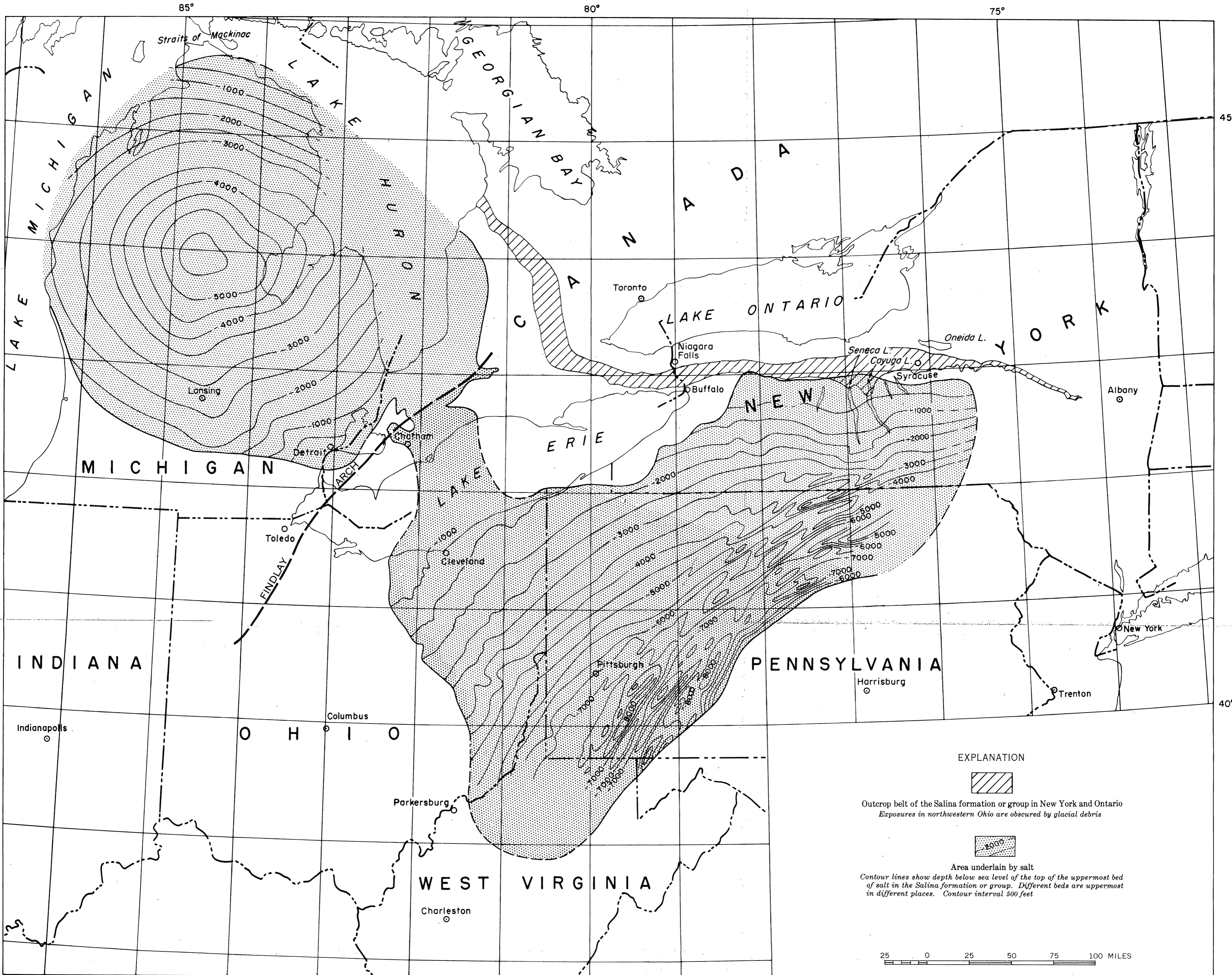
MAP SHOWING DEPTH BELOW SEA LEVEL OF TOP OF UPPERMOST SALT BED IN THE SALINA FORMATION OR GROUP
